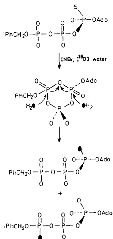
Scheme 2. The mechanism of displacement of sulphur from adenosine 5'-[(S)α-thio-γ-benzyl]triphosphate promoted by cyanogen bromide in [ 18 O]water.
