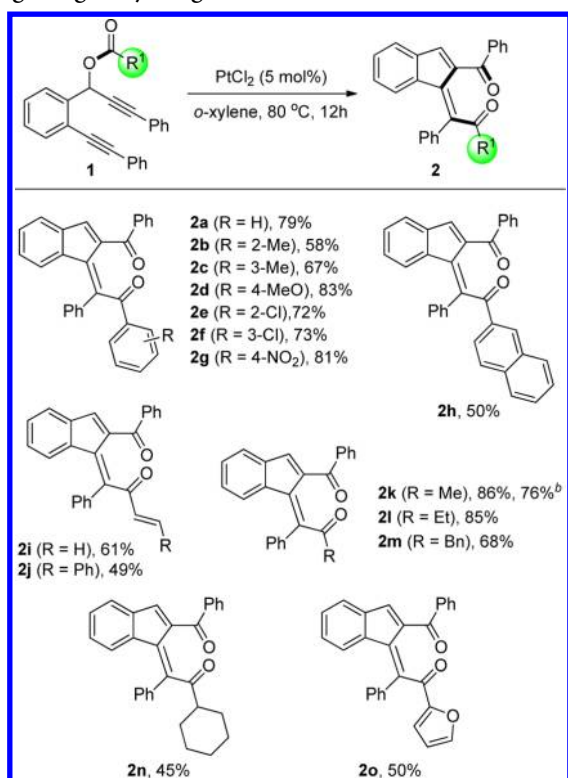
Scheme 3. Scope of the Acyl Group in the \text{PtCl}_2 -Catalyzed Long-Range Acyl Migration Reaction a
