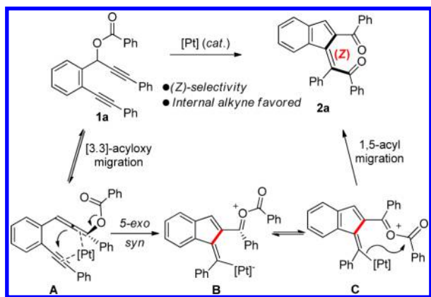
Scheme 2. Possible Mechanism for the Platinum-Catalyzed Pentannulation/Long-Range 1,5-Acyl Migration Reaction
