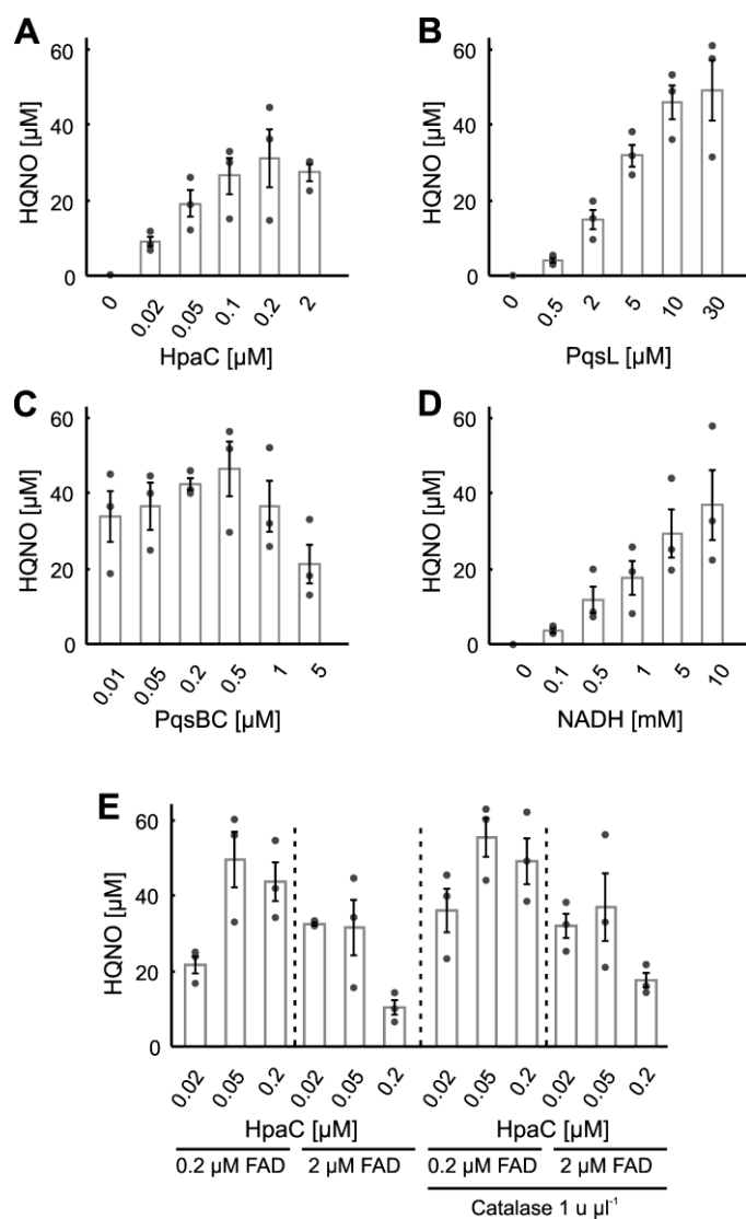
Figure 3. HQNO formation in the coupled PqsL/PqsBC reaction as a function of individual components of the assay. Reactions were run for 2 hours for complete conversion of PqsBC substrates before products HHQ (not shown) and HQNO were extracted with ethyl acetate and analyzed by HPLC. A , 5 μM PqsL was incubated with varying concentrations of the FAD reductase HpaC, 0.5 μM PqsBC and 100 μM 2-ABA, 120 μM octanoyl-CoA and 5 mM of NADH, B PqsL was varied, concentrations like in A, but with 0.2 μM HpaC, C variation of PqsBC shows that excess PqsBC depletes 2-ABA before conversion by PqsL, leading to a decrease in HQNO (conditions like A, but with 0.05 μM HpaC and 0.2 μM FAD), D variation of NADH illustrates the inefficiency of the reaction in vitro (conditions like in A, but with 0.2 μM HpaC), E supplementation with 0.2 μM FAD increases reaction efficiency and requires less HpaC for efficient HQNO formation (NADH was 5 mM). Excess of FAD (2 μM series) decreases the yields. To confirm that oxygen depletion by FADH 2 autooxidation was the cause of reduced product formation, the experiment was repeated with catalase supplementation (right side). Oxygen recovery out of H 2 O 2 by catalase leads to an increase of reaction efficiency. Error bars represent standard deviations.
