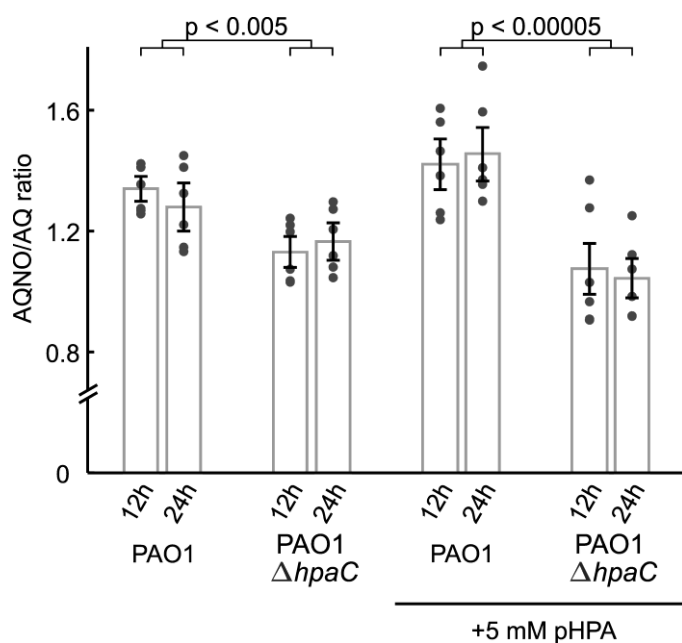
Figure 4. Impact of the deletion of hpaC on the production of AQ and AQNO. Pseudomonas aeruginosa strains PAO1 and PAO1 \Delta hpaC were cultivated in LB medium with 2 mM anthranilic acid at 37°C. AQ and AQNO were quantified by HPLC 12 hours and 24 hours after inoculation, and ratios between AQs and AQNOs were calculated. Supplementation of media with 5 mM p -hydroxyphenylacetic acid (pHPA, indicated) led to different effects in both strains. Error bars represent standard deviations.
