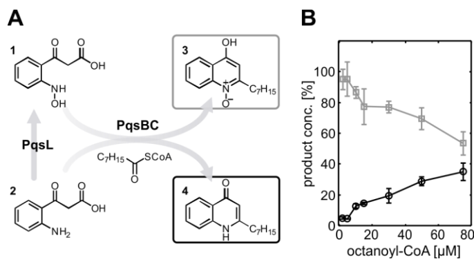
Figure 6. Substrate preference of PqsBC. A The reaction scheme on the left illustrates the two substrates 2-ABA (1) and 2-HABA (2); the latter being generated in situ by PqsL in the coupled PqsL-PqsBC reaction (additionally required substrates NADH, O_2 and the supporting enzyme HpaC were left out for clarity). Depending on its substrate preference, PqsBC converts either compound to the respective product (3 – HQNO, 4 – HHQ) until octanoyl-CoA is depleted. B The dependence on octanoyl-CoA reveals which substrate, 2-ABA or 2-HABA, is the preferred and/or more efficient one. Initial 2-ABA concentration was 250 \mu M , HQNO – grey, HHQ – black. Error bars reflect SEM out of three independent replicates.
