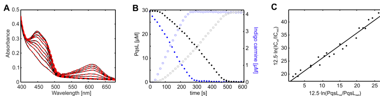
Figure 2. Midpoint potential of PqsL-bound FAD. A Representative spectra of the reduction of a PqsL/indigo carmine solution by xanthine oxidase. Black lines indicate real spectra, red lines correspond to composite spectra of least squares fitting using the PqsL and indigo carmine spectra shown in Fig. S1, and of reduced/oxidized benzyl viologen. B Reduction of PqsL and indigo carmine as calculated from the fitting (one representative experiment). Solid points reflect oxidized species, open points indicate reduced species concentrations (PqsL – black, indigo carmine – blue). C Nernst Plot comprising data collected in three independent experiments.
