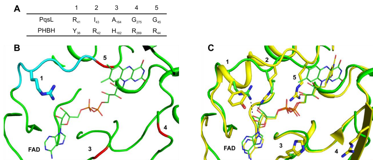
Figure 7 Structural investigation of cofactor and co-substrate binding in PqsL. A Survey of key residues for NADPH interaction in pHBH and corresponding residues of PqsL, as deduced from the structural alignment of PqsL with pHBH. B View of the 6FHO model (green) with the remodeled loop (cyan). Positions involved in NADPH recognition in pHBH that likely are dysfunctional in PqsL are highlighted in red: R 41 (1), which aligns with Y 38 of pHBH and adopted the function of R 42 (2) of pHBH (see C ) is shown in stick representation. C Close up of the flavin binding site of PqsL (green) aligned with pHBH (1PBE, yellow).
