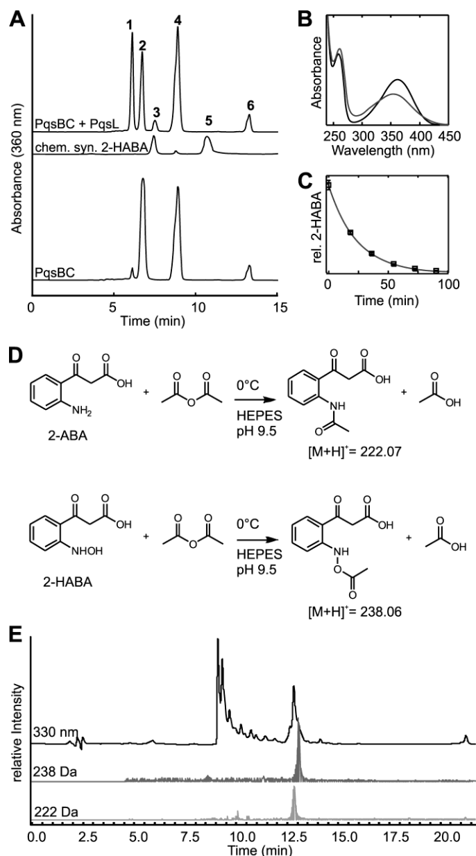
Figure 5. Identification of the PqsL reaction product 2-HABA. A The diagram shows chromatograms (stacked) of enzyme assays (top) and chemically synthesized (chem. syn.) 2-HABA (middle) from reverse phase HPLC. Control experiments (e.g. using PqsBC, bottom trace) and spectra comparisons (not shown) allow the assignment of peaks to 1 – NAD, 2 – NADH, 3 – 2-HABA, 4 – 2-ABA, 5 – 2-NBA, 6 – 2-AA. For confirmation of 2-HABA authenticity, peak 3 was prepared and converted with PqsBC to yield exclusively HQNO (not shown). B Comparison of normalized UV absorption spectra of 2-HABA (gray) and 2-ABA (black) as recorded with the HPLC diode array detector. C Decomposition of 2-HABA determined with HPLC. Error bars reflect standard error of mean (three representative replicates of synthetic and enzymatically prepared 2-HABA). Data were fitted with one exponential function (gray line) revealing a half-life of 16.2 \pm 0.1 min. D Reaction schemes of derivatizations of 2-ABA and 2-HABA with acetic anhydride. E LC-MS identification of the products of derivatization (according to D) of 2-ABA and of the of PqsL reaction products. Upper trace shows UV absorbance as measured with the LC-MS DAD detector, middle and lower traces show extracted ion chromatograms of the denoted masses of the positive MS.
