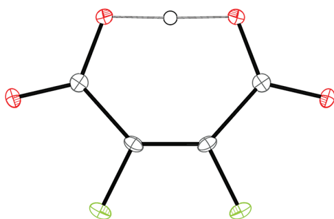
Figure 1. X-ray structure of hydrogen difluoromaleate monoanion in the crystal of its potassium salt.
