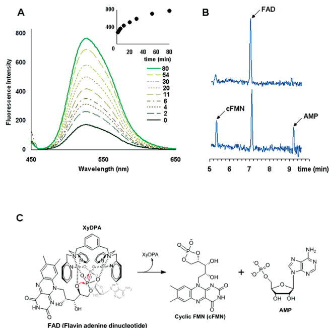
Figure 1. Catalytic splitting of FAD to cyclic FMN by XyDPA . (A) Fluorescence enhancement at 525 nm in the mixture of FAD (50 \mu M) and XyDPA (5 \mu M) with time. Inset graph: Y-axis, fluorescence intensity at 525 nm; X-axis, elapsed time. (B) Capillary electrophoresis electropherograms of a reaction mixture of FAD (100 \mu M) and XyDPA (10 \mu M) after 10 min (upper) and 1 h (lower) for FAD splitting catalyzed by XyDPA (10 \mu M) at pH 7.4 and 27 ^{\circ} C. (C) Proposed mechanism of FAD splitting to cFMN and AMP by XyDPA .
