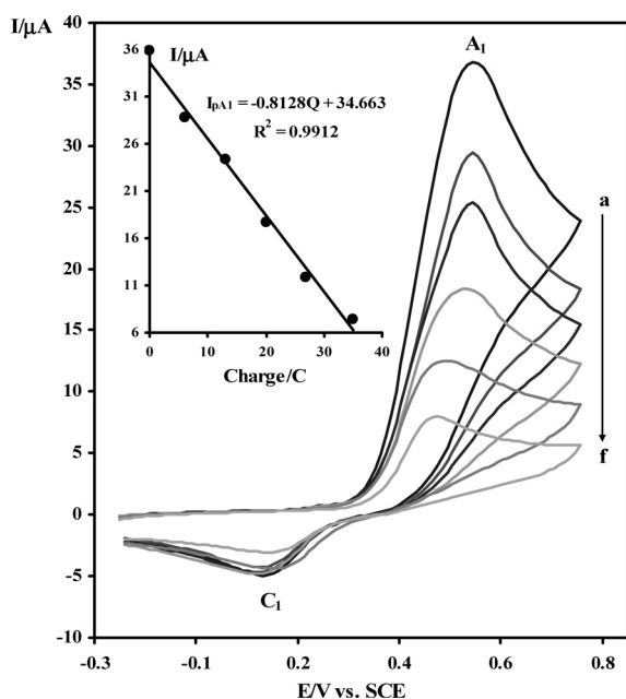
Fig. 6. Cyclic Voltammograms of 0.1 mmol 3,4-Dihydroxybenzaldehyde ( 1b ) in the Presence of 0.1 mmol 3-Hydroxy-1H-phenalene-1-one ( 3 ) at a Glassy Carbon Electrode during Controlled Potential Coulometry at 0.45 V versus SCE. After consumption of (a) 0, (b) 6, (c) 13, (d) 20 (e) 27, and (f) 35 C. Scan rate 100 \text{ mV s}^{-1} . Inset: variation of peak current ( I_{pA1} ) versus charge consumed. t = 25 \pm 1^\circ \text{C}
