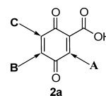
Fig. 3. The Structure of o -Benzoquinone 2a
