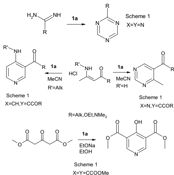
Scheme 2. Known reactions of 1,3,5-triazine ( 1a ) with 1,3-binucleophiles.
