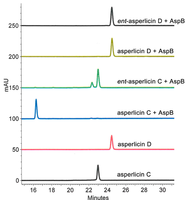
Figure 2. HPLC analysis (at 274 nm) of in vitro enzymatic reaction of AspB with enantiomeric pairs of asperlicin C and D.
