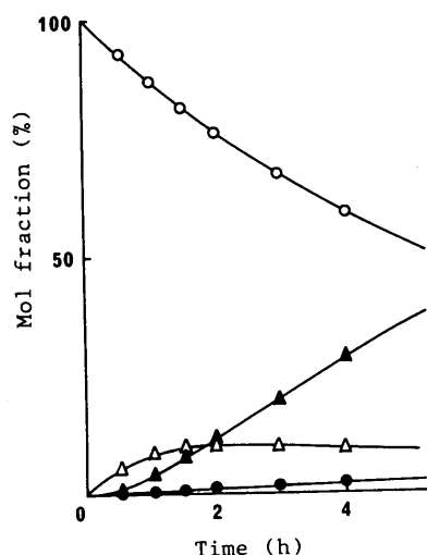
Fig. 2. Time Courses of \Delta^3 Ester Ia (○), \Delta^2 Ester IIa (△), \Delta^3 Acid IIIa (●) and \Delta^2 Acid IVa (▲) during the Degradation of POM Ester Ia
