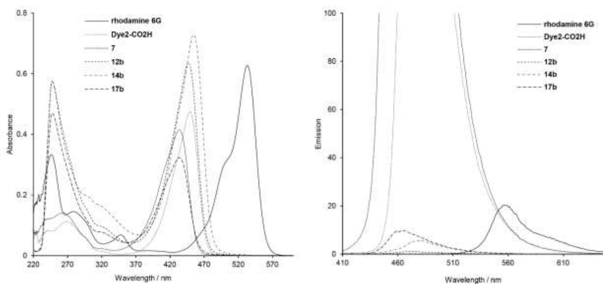
Figure 5. UV-Vis absorption (left) and emission spectra (right) of rhodamine 6G, Dye2-CO 2 H , intermediate 7 and the corresponding ester 12b and amide 14b , 17b conjugates, at 10 \mu M in CHCl 3 .
