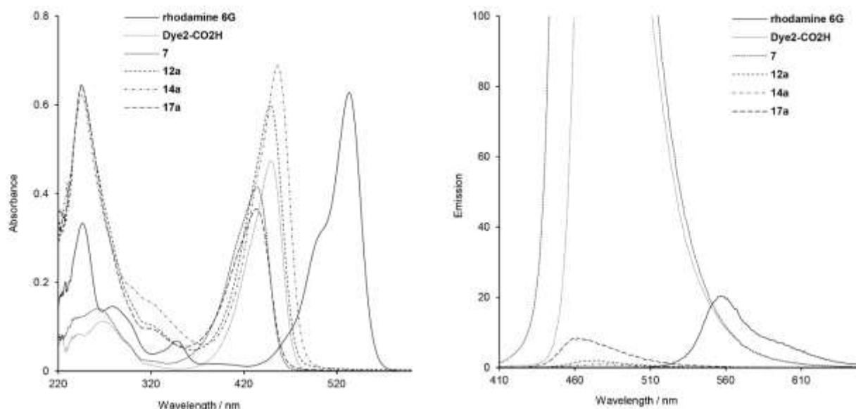
Figure 4. UV-Vis absorption (left) and emission spectra (right) of rhodamine 6G, Dye2-CO 2 H , intermediate 7 and the corresponding ester 12a and amide 14a , 17a conjugates, at 10 \mu M in CHCl 3 .
