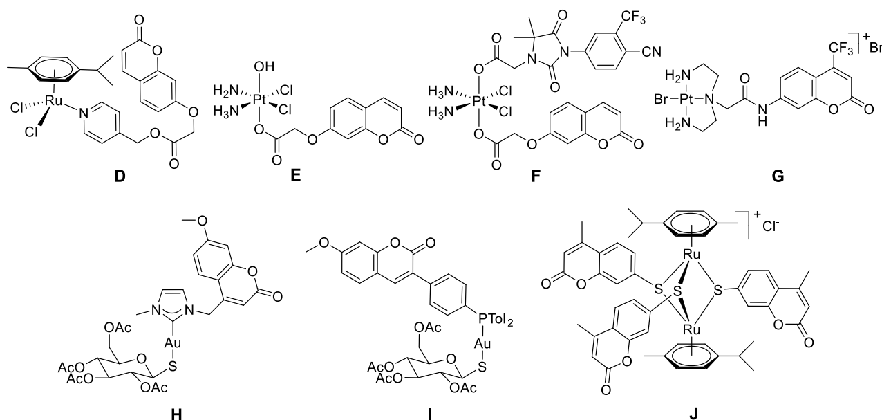
Figure 2. Structure of various organometallic moiety-coumarin conjugates.
