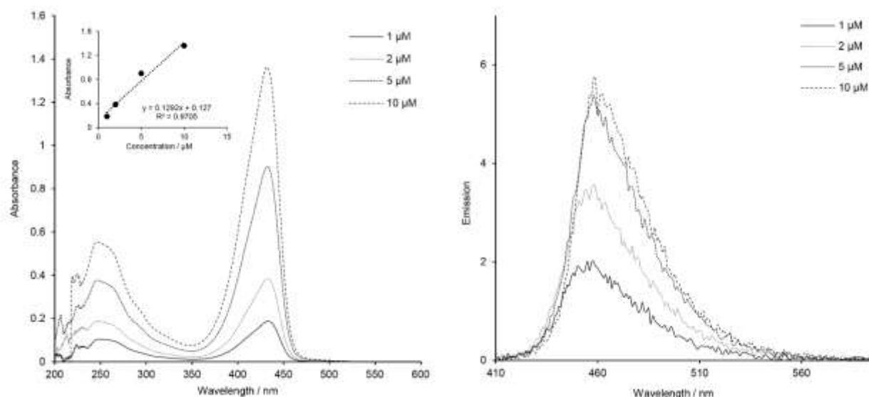
Figure 6. UV-Vis absorption (left) and emission spectra (right) of tri-coumarin ester conjugate 22 at various concentrations in \text{CHCl}_3 .
