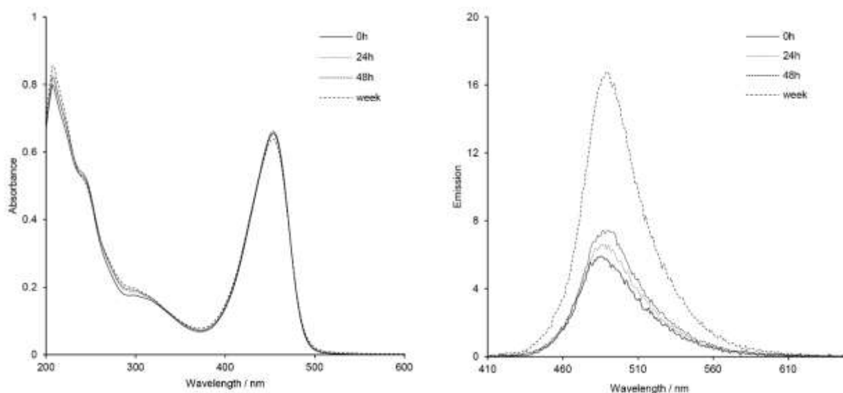
Figure 7. UV-Vis absorption (left) and emission spectra (right) of trithiolato ruthenium(II)- p -cymene complex 14b after 0 h, 24 h, 48 h, and one week (168 h) of exposure to indoor light at 10 \mu M in EtOH.
