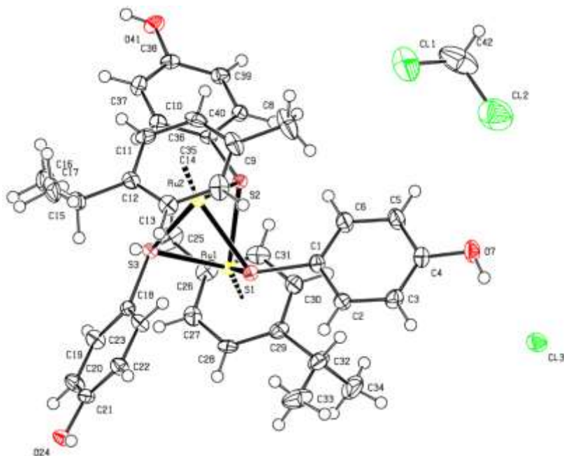
Figure 3. ORTEP representation of complex 21 (thermal ellipsoids are 50% equiprobability envelopes, and H atoms are spheres of arbitrary diameter; the asymmetric unit contains also one \text{CH}_2\text{Cl}_2 molecule).
