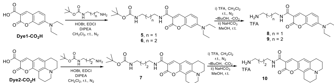
Scheme 2. Synthesis of the coumarin precursors containing an amino spacer 8 , 9 and 10 .
