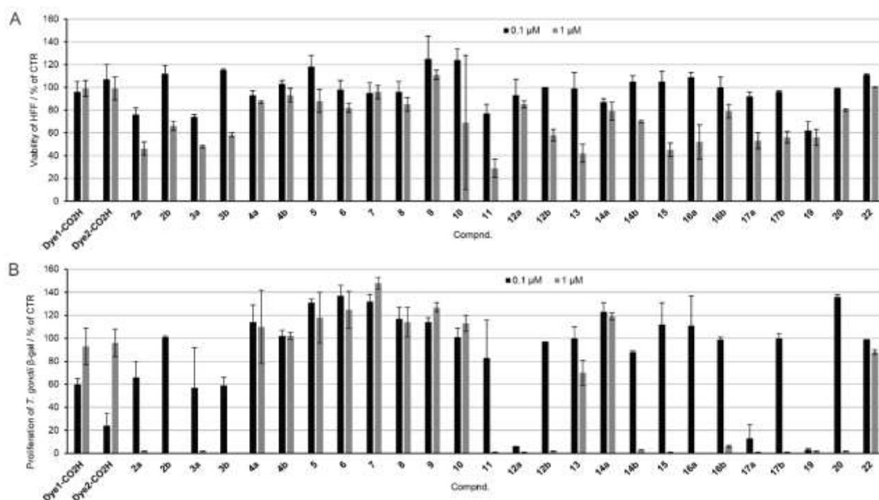
Figure 8. In vitro activities of all compounds at 0.1 \mu M and 1 \mu M on HFF viability (A) and T. gondii \beta -gal tachyzoites proliferation (B), in relation to treatments with 0.1% DMSO. For each assay, standard deviations were calculated from triplicates.
