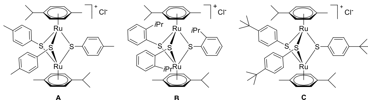
Figure 1. Structure of cationic trithiolato di-ruthenium(II)-arene complexes presenting high cytotoxicity against cancer cells and efficacy against various parasites.
