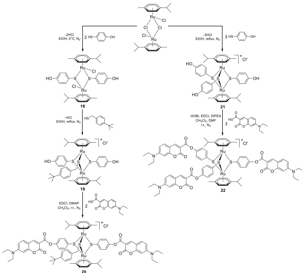
Scheme 5. Synthesis of conjugates 20 and 22 bearing two and, respectively, three fluorophore units.
