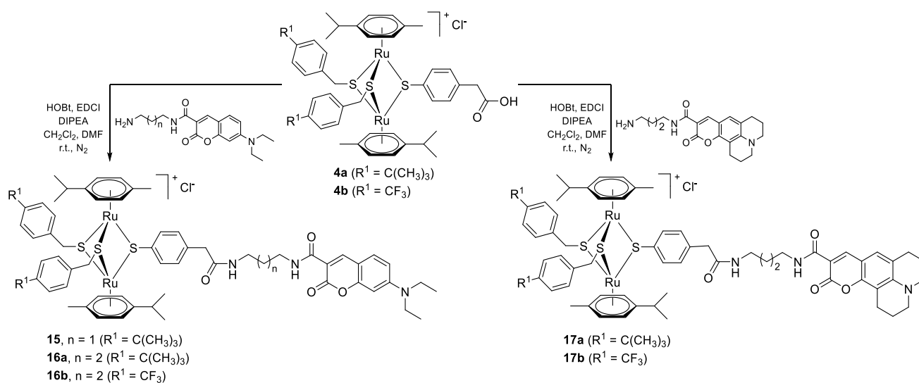
Scheme 4. Synthesis of the coumarin conjugates 15 , 16a/b and 17a/b containing an amino spacer.
