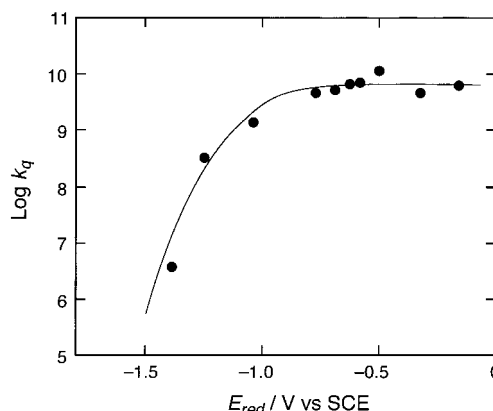
Figure 2. Rehm–Weller plot of the fluorescence quenching rate constant ( k_q ) in aqueous solution as a function of the reduction potential ( E_{\text{red}} ) of quencher. The solid curve is obtained from a best fit of experimental data to the Rehm–Weller empirical expression (see eqs 3–7).
