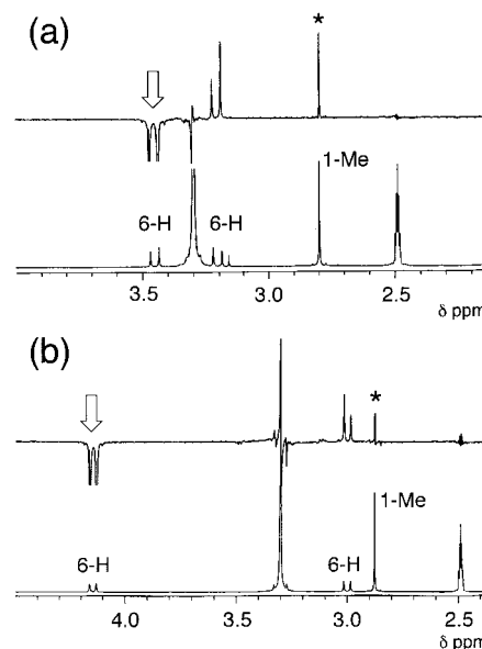
Figure 7. 400 MHz ^1\text{H} NMR spectra (lower trace) and NOE difference spectra (upper trace) of (a) 1a[meso] and (b) 1a[rac] in dimethyl sulfoxide- d_6 at 303 K. Arrows show irradiated H6 peaks.
