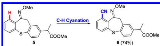
Scheme 1. Cyanation of Zaltoprofen Derivative 5 a
