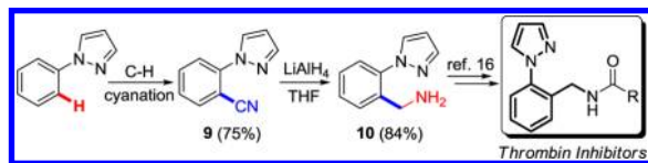
Scheme 3. Introduction of an Aminomethyl Group
