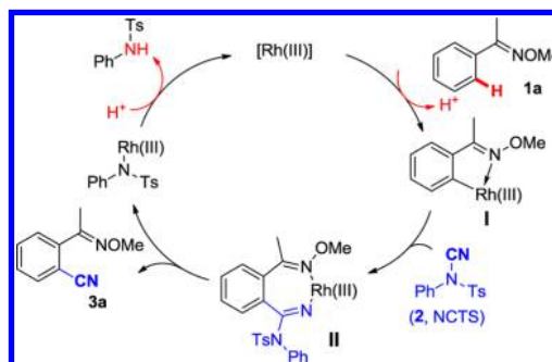
Figure 1. Proposed mechanism.
