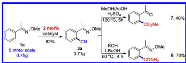
Scheme 2. A Larger-Scale C–H Cyanation Reaction
