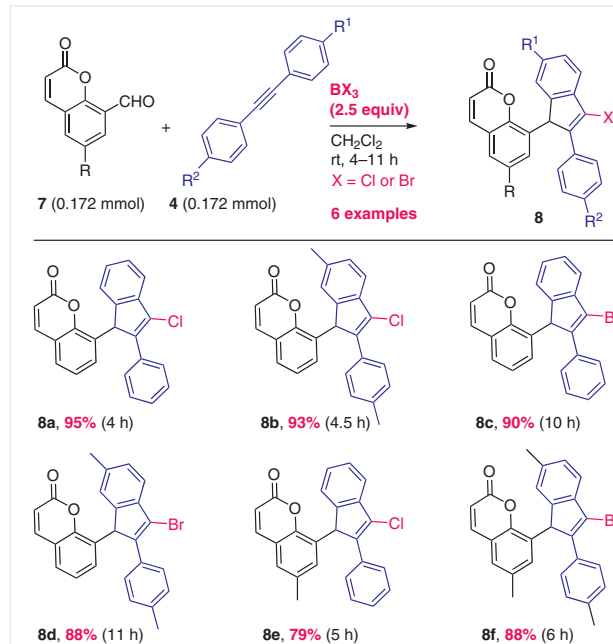
Scheme 6 Substrate scope for coumarin-based 3-halo-functionalized 1 H -indene synthesis. Reagents and conditions: 7 (0.172 mmol), 4 (0.172 mmol), BX 3 (2.5 equiv), CH 2 Cl 2 (2 mL), rt, 4–11 h. Isolated yields were recorded.
