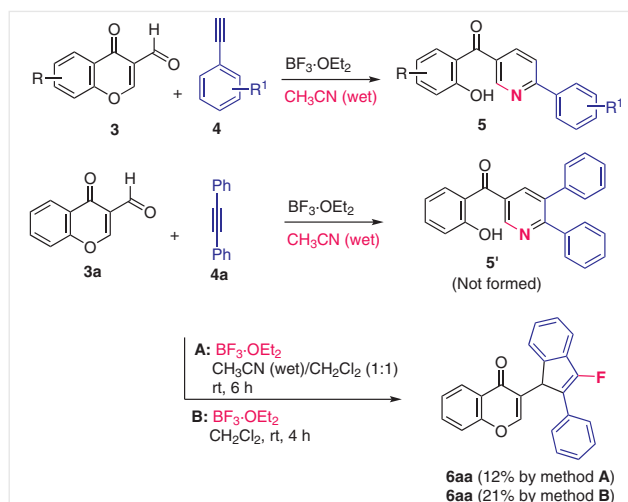
Scheme 2 Strategies for 2-arylpyridines and haloindenes
