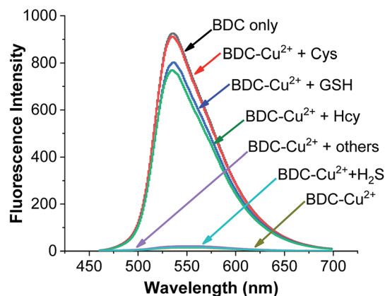
Fig. 8 Fluorescence spectra of BDC ( 5 \mu\text{M} ); \text{BDC (} 5 \mu\text{M)} + \text{Cu}^{2+} (5 \mu\text{M)} ; \text{BDC (} 5 \mu\text{M)} + \text{Cu}^{2+} (5 \mu\text{M)} + \text{Cys/Hcy/GSH/Ala, Asp, Arg, Gly, Glu, Ile, Leu, Lys, Met, Thr, Ser, Tyr, Trp, Val, His, and } \text{H}_2\text{S (} 10 \mu\text{M)} .
