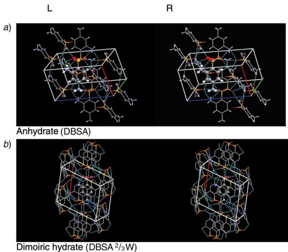
Fig. 4. Stereoviews of the unit cells of a) DBSA b) DBSA 2/3 W, c) DBSAHCl1, and d) DBSAHCl2. The view is on the best plane of the benzene ring with the sulfonate group on the vertical and the \text{NH}_2 group at C(2) to the left; the reference molecule is displayed as a ball-and-stick model. H-Atoms are omitted for clarity.
