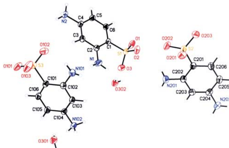
Fig. 3. ORTEP Diagram and atomic numbering of the three molecules of 2,4-diaminobenzenesulfonic acid and two molecules of water in the asymmetric unit of DBSA· \frac{3}{2} H 2 O
