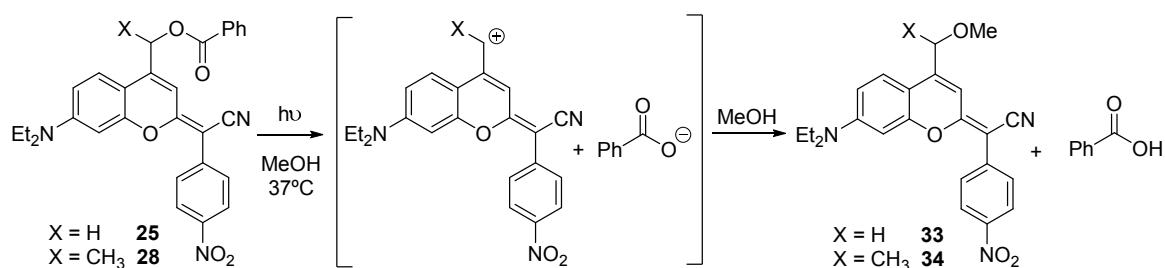
Scheme 5. Photolysis of coumarin derivatives 25 and 28 with green light.
