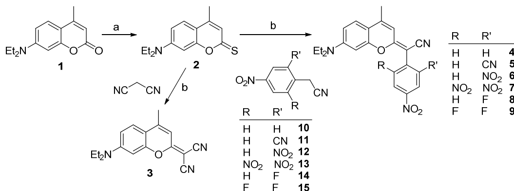
Scheme 2. Synthesis of coumarin-based chromophores 3-9 . a) Lawesson's reagent, toluene, 100°C, 12 h, 92%; b) Malononitrile or arylacetonitrile derivatives 10-15 , triethylamine, silver nitrate, anhydrous ACN, rt, 2-4 h, 86% ( 3 ), 40% ( 4 ), 54% ( 5 ), 68% ( 6 ), 27% ( 7 ), 42% ( 8 ), 55% ( 9 ).
