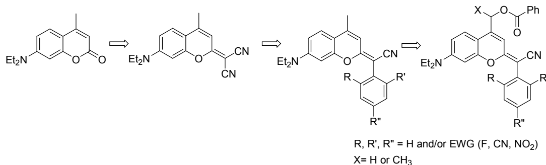
Scheme 1. Design of new coumarin-based chromophores and caging groups by replacement of a cyano group in dicyanocoumarin by a phenyl ring containing EWG at ortho and para positions.
