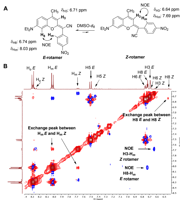
Figure 1. A) Structure of E and Z rotamers of compound 4 with some diagnostic NOE cross-peaks indicated. B) Expansion of the 2D NOESY spectrum ( t_m = 500 \text{ ms} , 25^\circ\text{C} ) of compound 4
