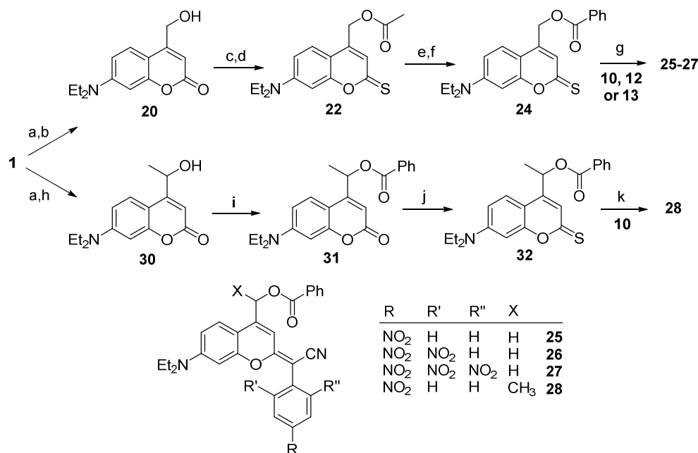
Scheme 4. Synthesis of caged model compounds 25-28 . a) SeO 2 , dioxane/H 2 O 1:0.03 (v/v), heat at reflux, 15 days, 40%; b) NaBH 4 , EtOH, 4 h, RT, 90%; c) AcOH, EDC·HCl, DMAP, DCM, 12 h, RT, Ar, 73%; d) Lawesson's reagent, toluene, 15 h, heat at reflux, 76%; e) HCl, EtOH, 20 h, 90°C; f) Benzoic acid, EDC·HCl, DMAP, DCM, 18 h, RT, Ar, 72% (2 steps e + f); g) first, arylacetonitrile derivatives 10 , 12 or 13 + NEt 3 in anhydrous ACN or ACN/DCM 1:1 2 h RT, then AgNO 3 2 h RT, 70% ( 25 ), 41% ( 26 ), 8% ( 27 ); h) CH 3 MgCl, anh. THF, 4 h, -78°C, 71%; i) Benzoic acid, EDC·HCl, DMAP, DCM, 18 h, RT, Ar; j) Lawesson's reagent, toluene, 15 h, heat at reflux, 69% (2 steps i + j); k) first, 10 + NEt 3 in anhydrous ACN/DCM 1:1 2 h RT, then AgNO 3 2 h RT, 69% ( 28 ).
