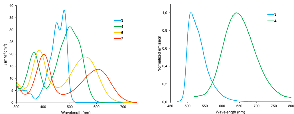
Figure 2. Comparison of the UV-vis spectra of selected coumarin derivatives 3 , 4 , 6 and 7 (left) and of fluorescence emission spectra of 3 and 4 (right) in DCM at RT.
