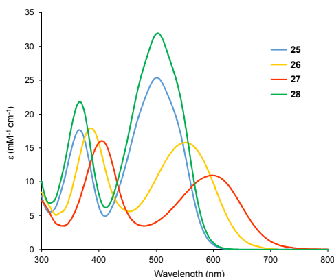
Figure 4. Comparison of the UV-vis spectra of coumarin derivatives 25-28 in DCM at RT.
