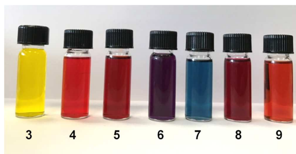
Figure 3. Photographic images of coumarin derivatives 3-9 in DCM under day light.
