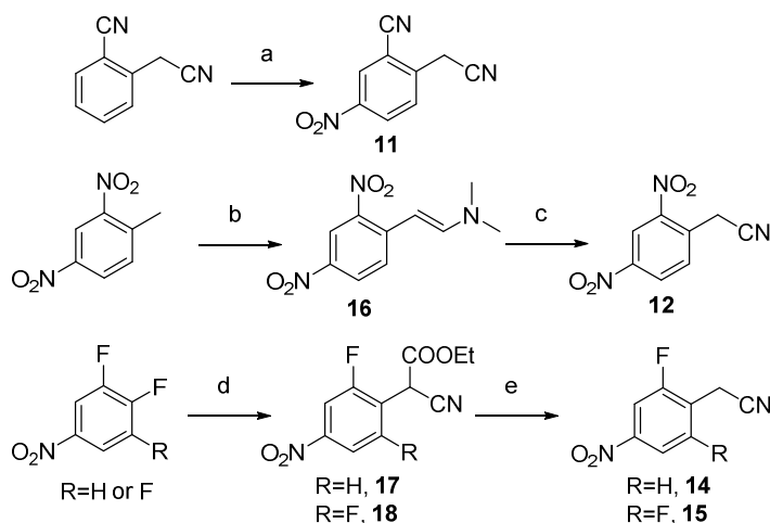
Scheme 3. Synthesis of arylacetonitrile derivatives 11-12 and 14-15 . a) \text{HNO}_3 , \text{H}_2\text{SO}_4 , -5^\circ\text{C} , 3 h, 60% ( 11 ); b) N,N -dimethylformamide dimethylacetal, anhydrous DMF, heat at reflux ( 16 ), 15 h, Ar atmosphere, 96% ( 16 ); c) hydroxylamine hydrochloride, formic acid, heat at reflux, 5 h, 60% ( 12 ); d) ethyl cyanoacetate, \text{K}_2\text{CO}_3 , KI, anhydrous DMF, 16 h at rt and 2 h at 100^\circ\text{C} , 98% ( 17 ), 72% ( 18 ); e) HCl, AcOH, 12 h, 100^\circ\text{C} , 32% ( 14 ), 39% ( 15 ).
