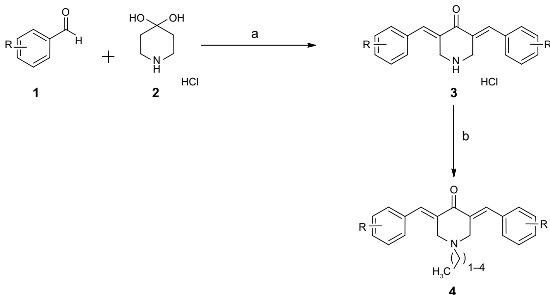
Figure 2 Synthesis of curcumin-inspired derivative.
