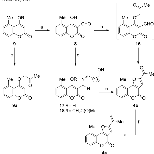
Scheme 4. Reagents and conditions: a) \text{MgCl}_2 (anh.), \text{Et}_3\text{N} , (\text{CH}_2\text{O})_n , THF, 50^\circ\text{C} , 1 h ( 8 , 87%); b) \text{ClCH}_2\text{COCH}_3 , \text{Al}_2\text{O}_3 , \text{CH}_2\text{Cl}_2 , 40^\circ\text{C} , 72 h ( 4b , 88%); c) \text{ClCH}_2\text{COCH}_3 , \text{K}_2\text{CO}_3 , DMF, 65^\circ\text{C} , overnight (50%); d) \text{H}_2\text{N}(\text{CH}_2)_4\text{CH}_2\text{OH} , PhMe, 90^\circ\text{C} , 1 h ( 8 , 85%); e) \text{ClCH}_2\text{COCH}_3 , \text{K}_2\text{CO}_3 , DMF, 65^\circ\text{C} , overnight (15%); f) \text{Ph}_3\text{PMe}^+\text{I}^- , \text{K}^+\text{BuO}^- , LiCl, THF, rt, 1 h ( 4a , 58%; 4b , 25%; 4a , 78%, based on recovered starting material).
