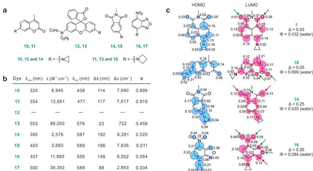
Figure 2. (a) Molecular structures of 10—17. (b) Experimental spectroscopic data for 10–17 in aqueous solution. \lambda_{\text{abs}} , peak UV—vis absorption wavelength; \epsilon , molar extinction coefficient; \lambda_{\text{em}} , peak emission wavelength; \Delta\lambda and \Delta\nu , the Stokes shift; \phi , quantum yield. (c). The atomic contributions to the HOMO (highest occupied molecular orbital) and LUMO (lowest unoccupied molecular orbital) electron densities of 1, 10, 14 and 16, calculated based on the optimized molecular structures in the S_0 state. The blue/pink circle size represents the atomic contribution; only contributions greater than 0.02 are shown. Hydrogen bond formation sites in naphthalimide, coumarin, phthalimide, and NBD fluorophore scaffolds are indicated by arrows. Molecular sites that experience significant partial charge increase upon photoexcitation are highlighted by red arrows in 14 and 16.
