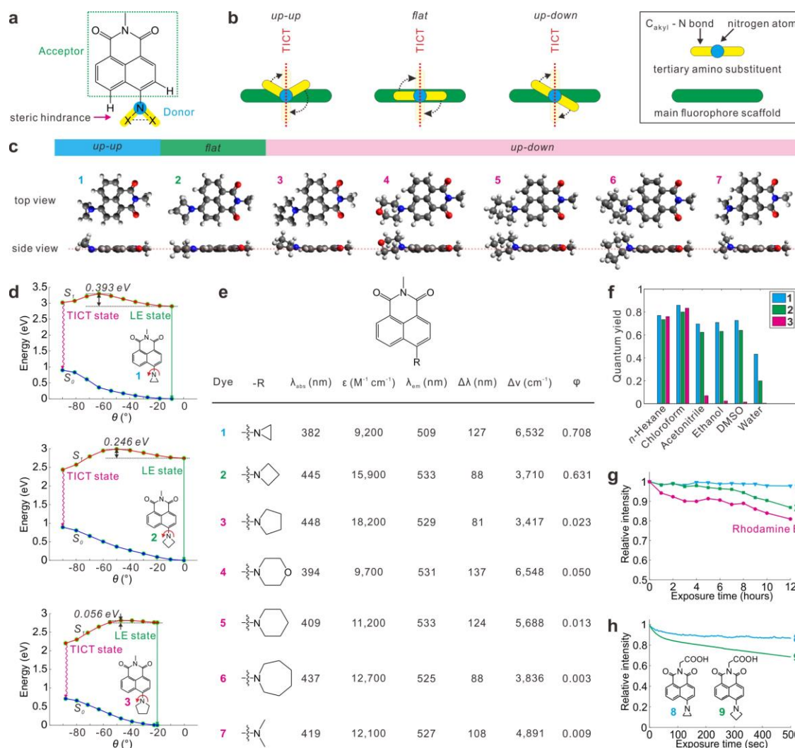
Figure 1. The three-membered aziridine ring enhances the brightness and photostability of naphthalimide fluorophores. (a) Illustration of steric hindrance between donor and acceptor moieties of a fluorophore. (b) Three types of alignment conformations between the two amino “arms” (highlighted in yellow) and the main fluorophore scaffold (green) in the ground state ( S_0 ). Arrows indicate potential rotations to enter the twisted intramolecular charge transfer (TICT) state in the first excited state ( S_1 ). (c) The top and side views of the theoretically optimized molecular structures of 1–7 in ethanol in the ground state. (d) Calculated potential energy surfaces (PES) of the ground ( S_0 , in blue) and the first excited singlet ( S_1 , in red) states of 1–3 in ethanol, as a function of the rotational angle ( \theta ) between the amino substituent and the main fluorophore scaffold. \theta is the average dihedral angle of two amino “arms” with respect to the naphthalimide scaffold. The LE state has a more planar conformation and less charge transfer compared to the TICT state. (e) Experimental spectroscopic data for 1–7 in ethanol. \lambda_{\text{abs}} , peak UV–vis absorption wavelength; \epsilon , molar extinction coefficient; \lambda_{\text{em}} , peak emission wavelength; \Delta\lambda and \Delta\nu , the Stokes shift; \phi , quantum yield. (f) Experimental quantum yields of 1–3 in various solvents. (g) Relative intensity changes of 1, 2, and Rhodamine B in DMSO/water mixture (volume ratio, 30:70) during 12 hours of strong white light exposure. (h) Relative intensity changes of 8 and 9 in water during 500 seconds of strong laser radiation (416 nm) in microfluidic channels. The insets show the molecular structures of 8 and 9.
