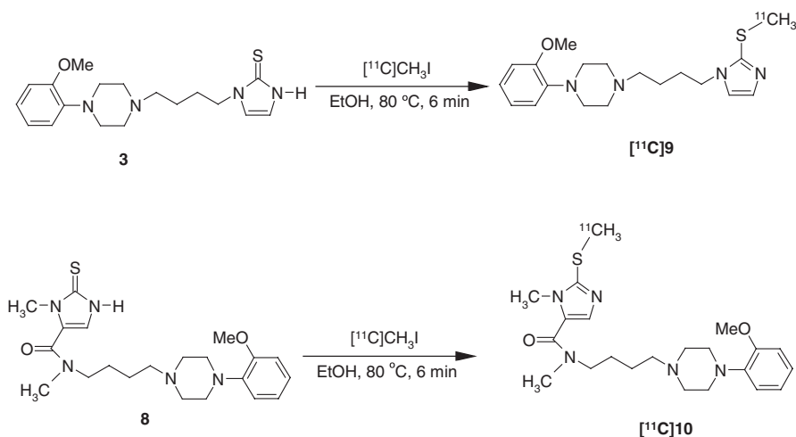
Scheme 5. Radiosynthesis of [ 11 C]9 and [ 11 C]10
