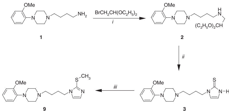
Scheme 3. Synthesis of the labelling precursor 3 and reference compound 9 : (i) \text{K}_2\text{CO}_3 , acetonitrile, reflux, 48 h; (ii) KSCN, HCl 2 N, ethanol, reflux, overnight; (iii) NaOH, \text{CH}_3\text{I} , ethanol, rt, 3 h
