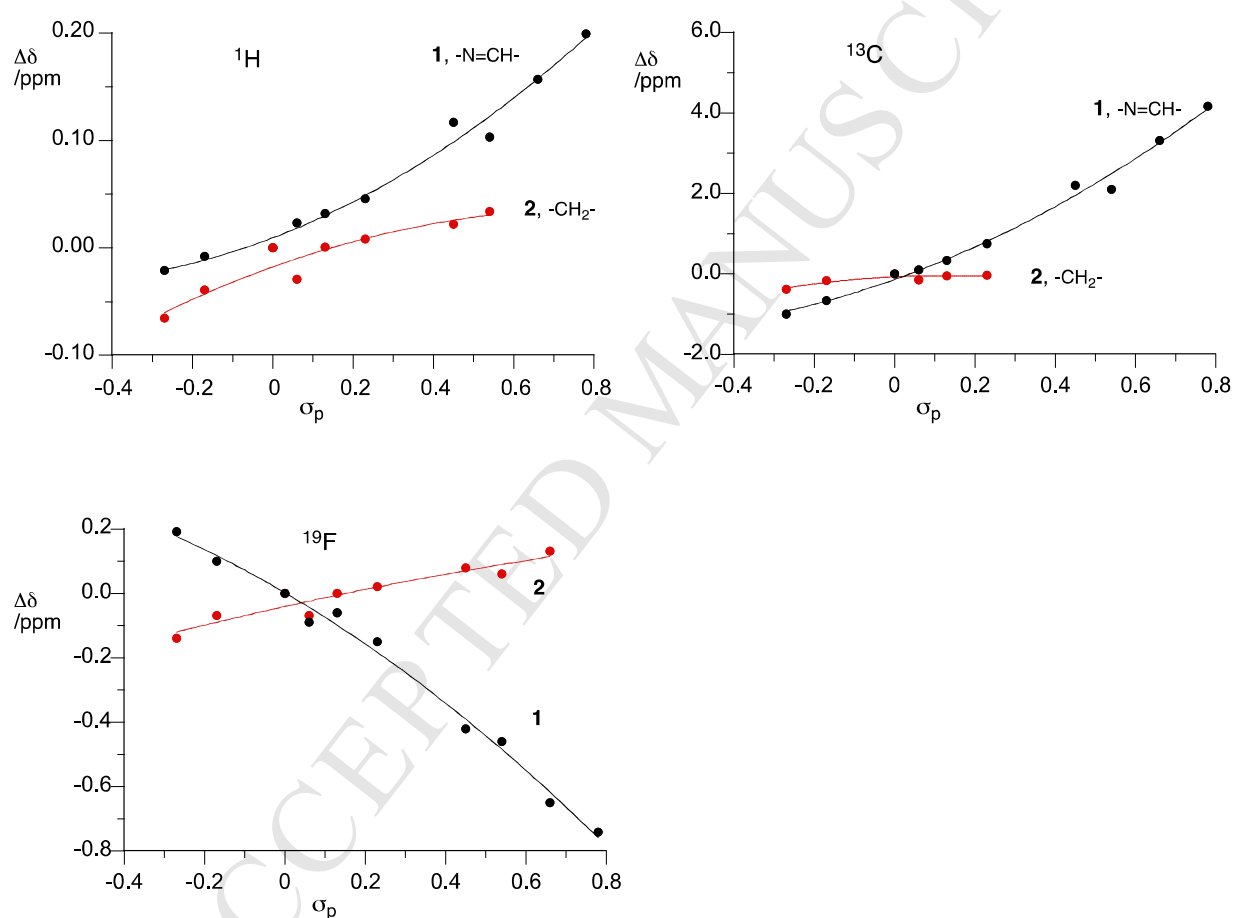
Figure 6. Correlation of the difference in ^1\text{H} , ^{13}\text{C} , and ^{19}\text{F} chemical shifts ( \Delta\delta = \delta_x - \delta_H ) for series of hydrazones 1 (black) and azo derivatives 2 (red).
