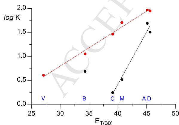
Figure 10. A plot of experimental (black) and theoretical data (red) for \log(K) of 1c–2c vs solvent parameter E_{\text{T}(30)} : V–vacuum, B–benzene, C–chloroform, M–methylene chloride, A–acetonitrile, D–dimethyl sulfoxide. Best fit line: experimental without B, \log K_{\text{exp}} = 0.218 \times E_{\text{T}(30)} - 8.32 , r^2 = 0.97 ; theoretical \log K_{\text{theor}} = 0.076 \times E_{\text{T}(30)} - 1.49 , r^2 = 0.988 .
