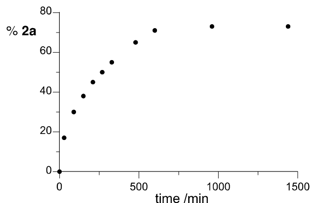
Figure 4. Formation of azo 2a in a \text{CDCl}_3 solution at ambient temperature by tautomerization of the hydrazono form 1a .
