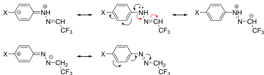
Figure 7. Selected resonance structures for 1 and 2 .
