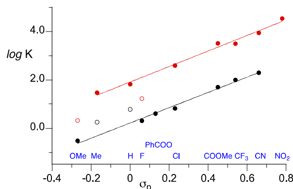
Figure 8. A plot of experimental (black) and calculated (red) equilibrium constants K for 1–2 against substituent parameter \sigma_p . Best fitting lines without the open-circle datapoints: \log K_{\text{exp}} = 3.15 \times \sigma_p + 0.22 , r^2 = 0.99 ; \log K_{\text{theor}} = 3.21 \times \sigma_p + 1.91 , r^2 = 0.99 .
