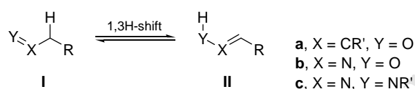
Figure 1. Tautomeric equilibria I–II for carbonyl ( a ), nitroso ( b ), and azo ( c ) compounds.
