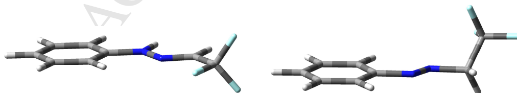
Figure 9. Molecular geometry for 1d (left) and 2d (right) obtained at the M06-2x/6-31G(2d,p) level of theory.
