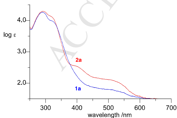
Figure 5. Electronic absorption spectra for 1a (blue) and 2a (red) in \text{CH}_3\text{CN} .
