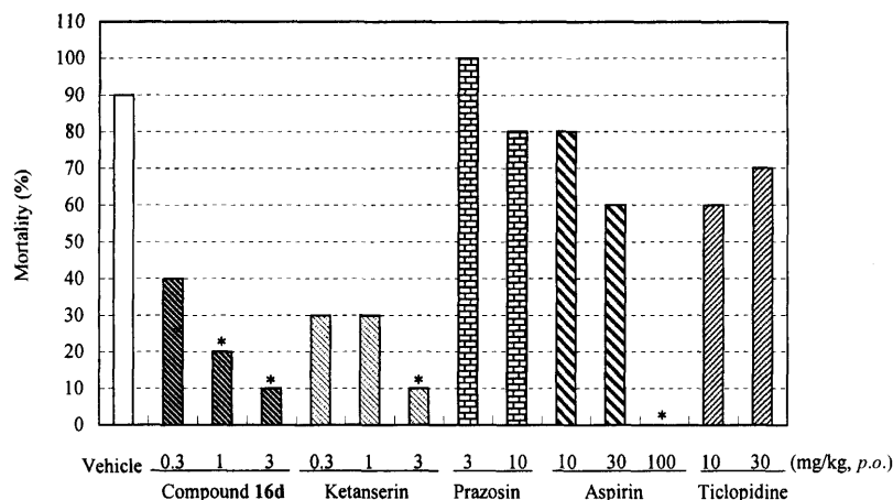
Fig. 4. Effects of Compound 16d , Ketanserin, Prazosin, Aspirin and Ticlopidine on Pulmonary Thromboembolic Death in Mice
