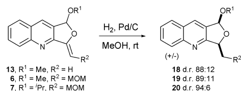
Scheme 4 Reduced furoquinolines 18–20 .
