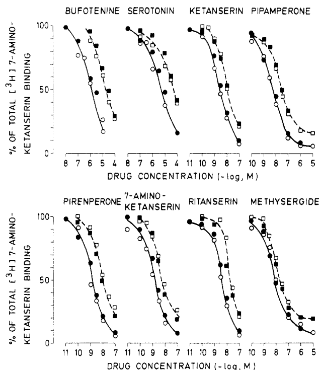
Figure 3. Displacement of [ ^3\text{H} ]-7-aminoketanserin binding to an (M + L + P) fraction (—) and a CHAPS/salt-solubilized (---) preparation from rat frontal cortex by different serotonin antagonists and agonists. Binding experiments were performed as described in the Experimental Section. [ ^3\text{H} ]-7-Aminoketanserin was used as 1 nM (M + L + P) or 2 nM (solubilized) final concentration. Filled and open symbols represent the results from two independent experiments, each performed in triplicate.
