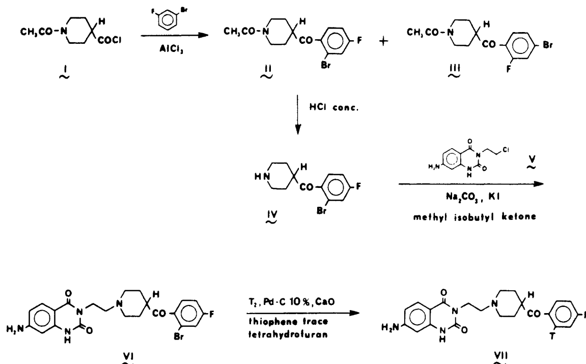
Figure 1. Synthesis of [ 3 H]-7-aminoketanserin.
