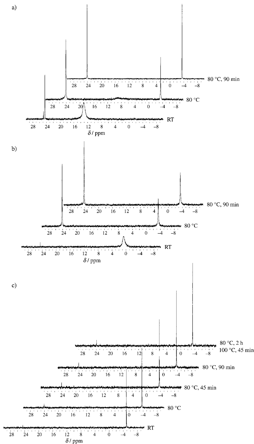
Figure 2. ^{31}\text{P} NMR spectra of the oxidative addition of [\text{Pd}(\text{PPh}_3)_4] to 4-bromobenzotrifluoride in the presence of different amounts of n\text{Bu}_4\text{NCN} : a) without added cyanide; b) in the presence of one equivalent of cyanide; c) in the presence of five equivalents of cyanide.
