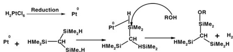
SCHEME 1 Proposed mechanism for the alcoholysis reaction of (\text{HMe}_2\text{Si})_3\text{CH} .
