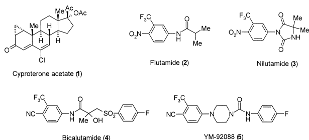
Fig. 1. Structures of Androgen Antagonists
