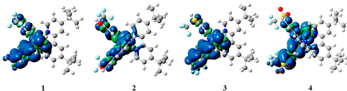
Figure 7. Triplet spin density distributions of complexes 1–4, obtained from DFT [(UB3LYP/SBKJC-VDZ for Ir(III)) and (6-31g** for C,H,N, (O),F,(S))] with CPCM(MeCN). Contours are isovalued at 0.02.
