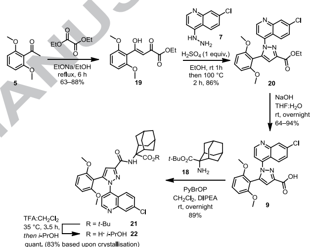
Scheme 5. Improved synthesis of Meclinertant (SR 48692, 2 ).
