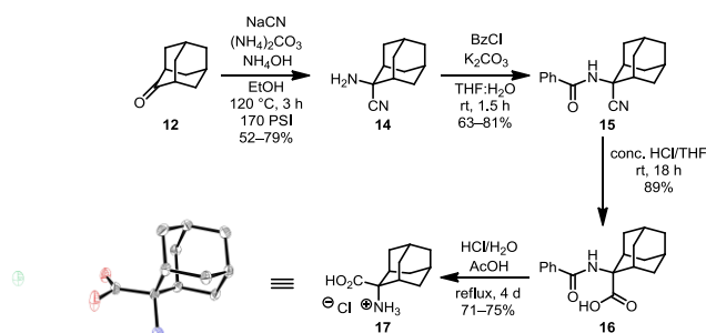
Scheme 3. Alternative route to the amino acid 17 .
