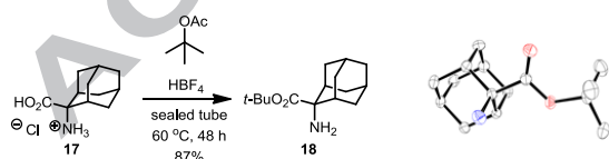
Scheme 4. tert -Butyl protection of amino acid 17 .
