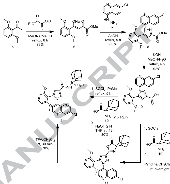
Scheme 1. Routes towards SR 48692 ( 2 ) reported by Sanofi-Aventis. 22,27
