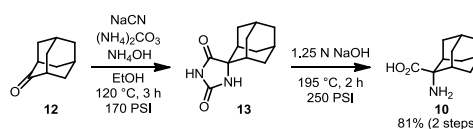
Scheme 2. Preparation of amino acid 10 via Nagasawa's route. 28
