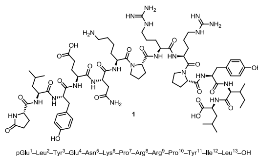
Figure 1. Neurotensin ( 1 ) and its linear amino acid sequence.
