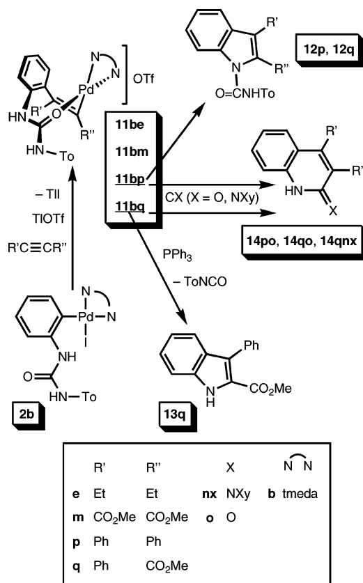
Scheme 4
