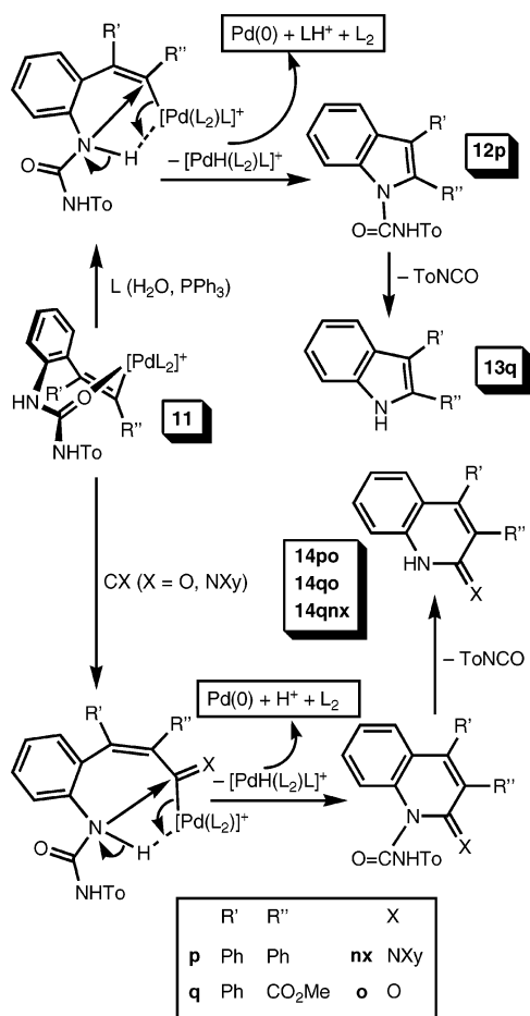
Scheme 5
