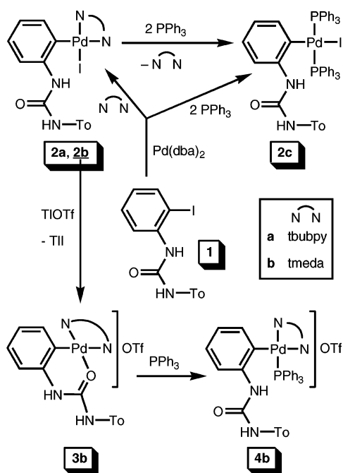
Scheme 1
