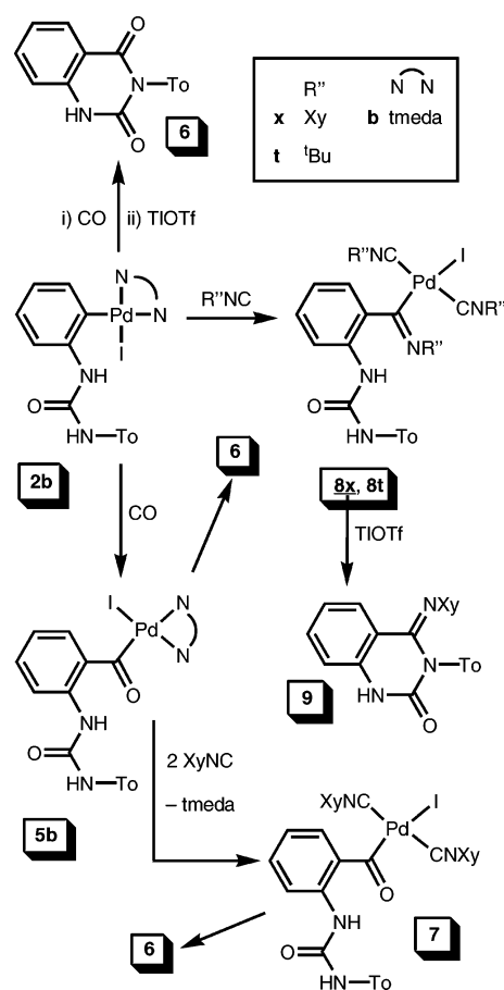
Scheme 2
