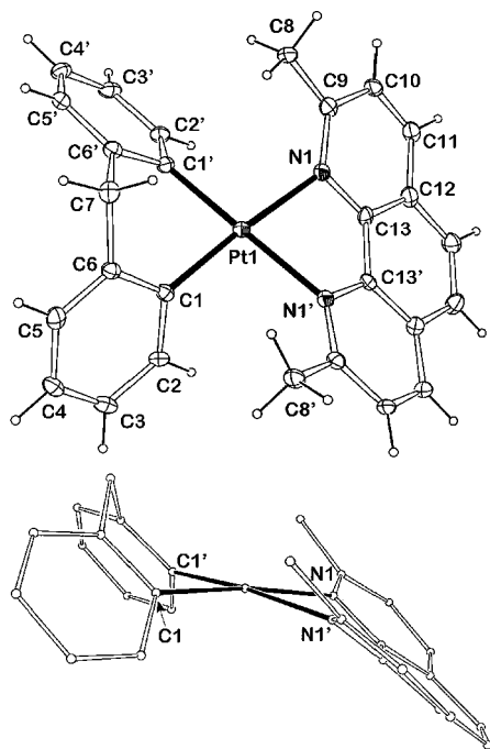
Figure 5. Molecular structure of [\text{H}_2\text{C}(\text{C}_6\text{H}_4)_2]\text{Pt}(2,9\text{-dimethyl-1,10-phenanthroline}) ( 14 ). In addition to a thermal ellipsoid plot (top, 30% probability; hydrogens as spheres of arbitrary radius), a ball-and-stick plot (bottom, hydrogens omitted for clarity) is shown in order to highlight the geometry of the six-membered chelate ring. The molecule has crystallographic mirror symmetry (mirror plane through C7, Pt1, and the center between N1 and N1'). Selected distances and angles ( \text{\AA} , deg): Pt1–C1, 1.999(5); Pt1–N1, 2.130(5); C1–Pt1–C1', 83.9(3); N1–Pt1–N1', 78.1(2); C1–Pt1–N1', 98.7(2); C1–Pt1–N1, 173.6(2); arenes in the metallacyclic ring are not coplanar: dihedral angle between best plane through C1–C2–C3–C4–C5–C6 and best plane through C1'–C2'–C3'–C4'–C5'–C6', 67.6(3); boat conformation of the metallacyclic ring: dihedral angle between plane through C1–Pt1–C1' and plane through C6–C7–C6', 86.0(6).
