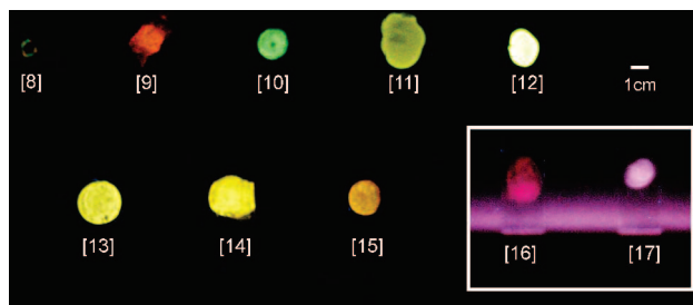
Figure 11. Room-temperature luminescence, caused by 365 nm excitation, from powder samples (thin layer) of compounds 8 – 17 . Regarding apparent relative intensities: layer thickness was not uniform and the brightness/contrast of the relatively weakly emitting (very thin layer) sample 8 was enhanced relative to 9 – 15 . Blue specks due to luminescence of the edges of the supporting glass slides were removed from the picture. The photograph of samples 16 and 17 , shown in the inset, was taken with the UV lamp very close (violet strip caused by excitation light).
