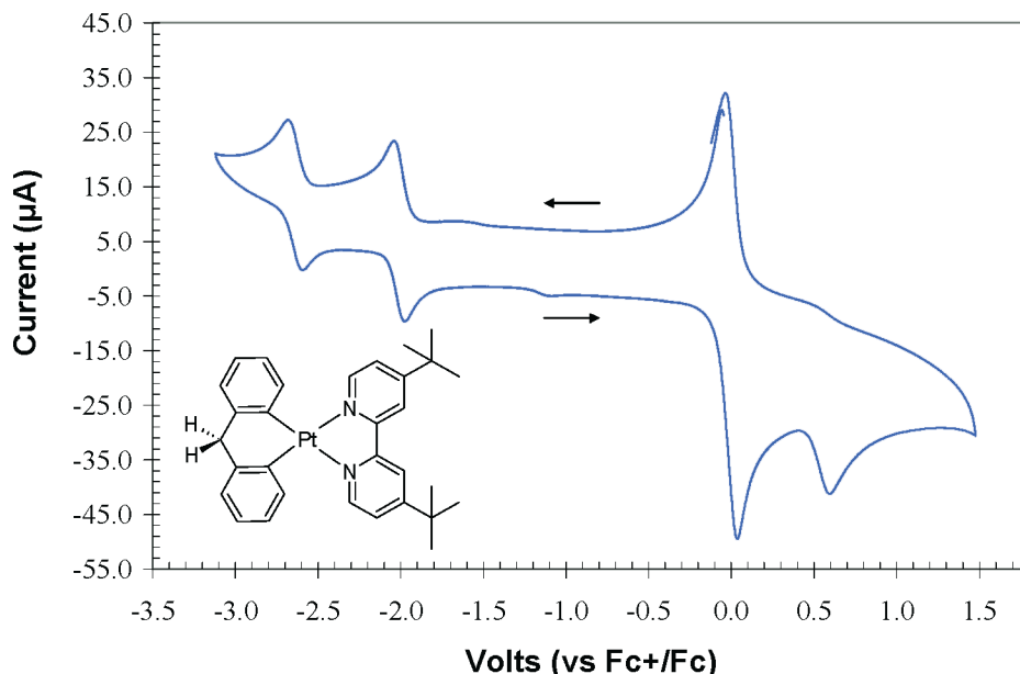
Figure 9. Cyclic voltammogram (CV) of 12 , measured in acetonitrile at 28 °C. Potentials are referenced relative to internal \text{Fc}/\text{Fc}^+ (defined as 0 V). Scan rate is 1000 mV/s. TBAHFP (0.1 M) was used as the supporting electrolyte.
