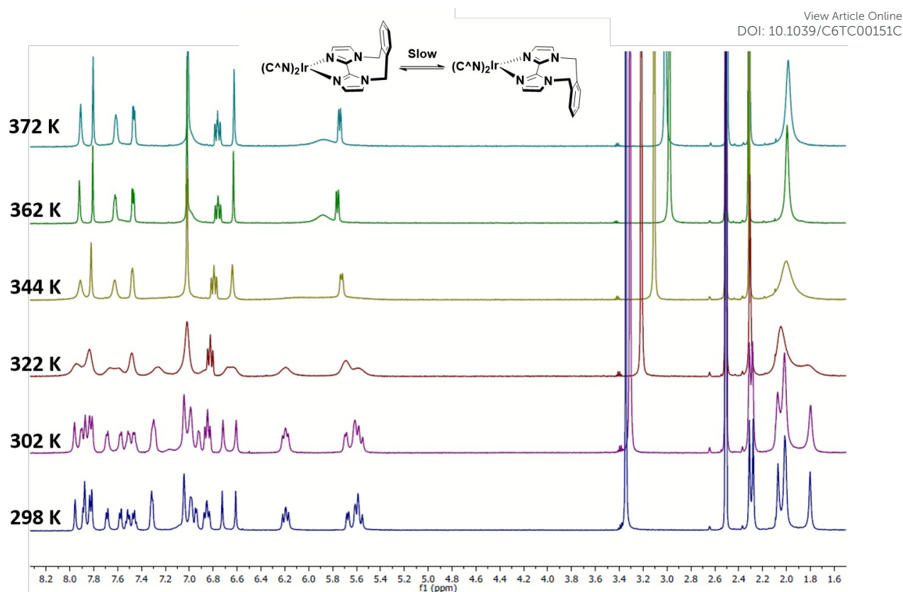
Figure 3. ^1\text{H} NMR temperature study of 3 in \text{DMSO}-d_6 from room 298 K to 372 K.
