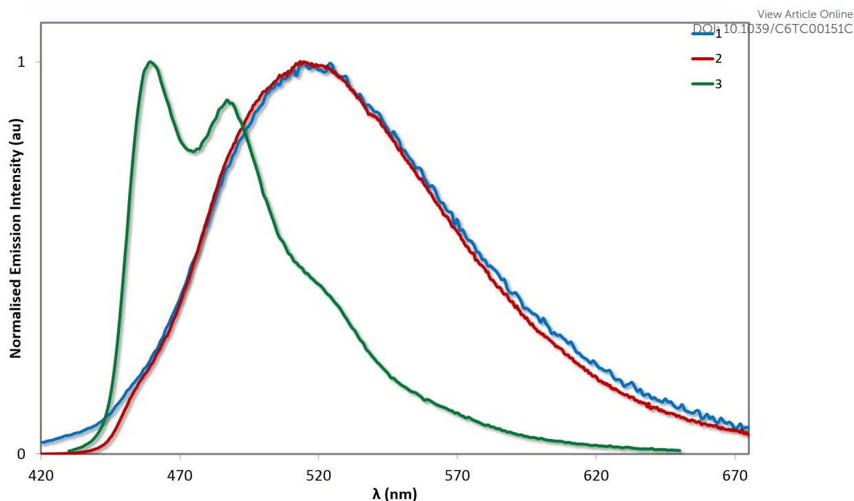
Figure 8. Normalised emission spectra for complexes 1-3 in deaerated MeCN solution. \lambda_{\text{exc}} : 360 nm.
