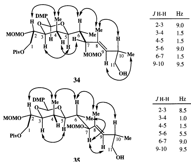
Fig. 4. NOESY Correlations and Coupling Constants of 34 and 35
