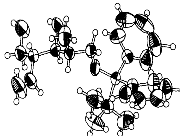
Fig. 2. X-Ray Crystal Structure of 13
