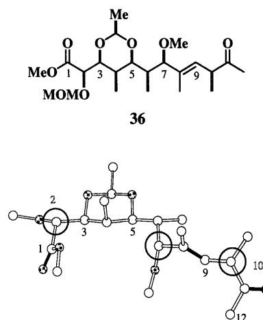
Fig. 5. The Most Stable Conformer of 36 Calculated by MM2-CONFLEX-3
