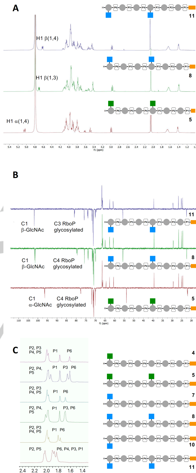
Figure 3. Characterization of the synthetic WTA-fragments. A) ^1\text{H} -NMR (500 MHz, \text{D}_2\text{O} ) of 5 , 8 and 11 . B) ^{13}\text{C} -NMR (126 MHz, \text{D}_2\text{O} ) of 5 , 8 and 11 . C) ^{31}\text{P} -NMR (202 MHz, \text{D}_2\text{O} , 10 mg/mL, pH 7) of 4 , 5 , 7 , 8 , 10 and 11 .
