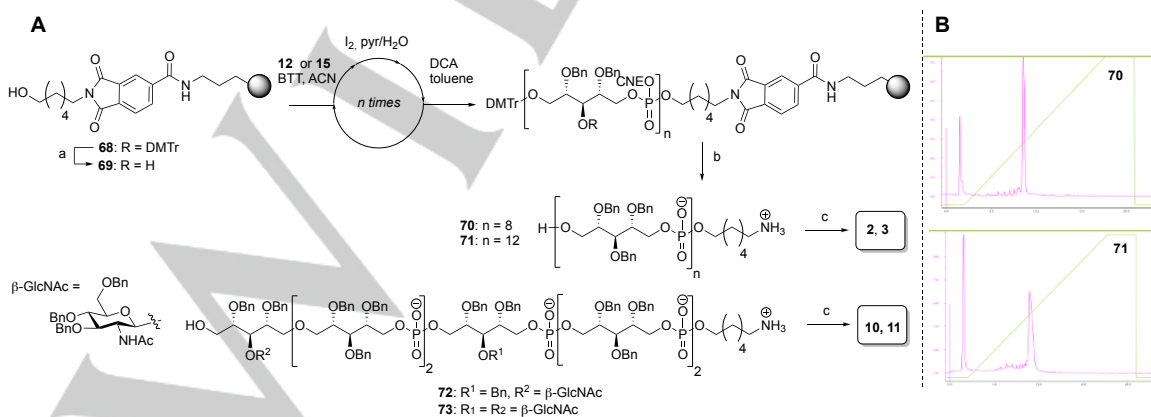
Scheme 3. Automated solid phase assembly of WTA-fragments. Reagents and conditions: a) 3% DCA in toluene (3 min); 12 or 15 BTT, ACN (5 min); \text{I}_2 , pyr/ \text{H}_2\text{O} (1 min); \text{Ac}_2\text{O} , N -methylimidazole, 2,6-lutidine, ACN (0.2 min); b) 25% \text{NH}_3 (aq) (60 min); 70 : 15%; 71 : 11%; 72 : 20%; 73 : 11%; c) Pd black, \text{H}_2 , dioxane \text{H}_2\text{O} , AcOH, 2 : 100%; 3 : 100%; 10 : 87%; 11 : 100%.
