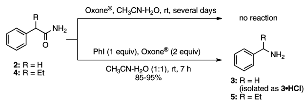
Scheme 2. Formation of Benzylamines by Hofmann Rearrangement of Carboxamides using Oxone
