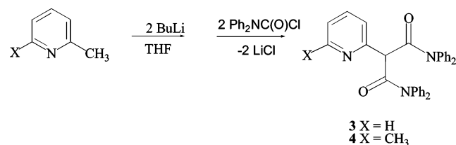
FIGURE 2. Molecular structure and atom labeling scheme for 4 . 39
