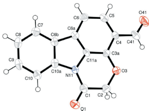
FIG. 1 ORTEP drawing of crystal structure of 4a
