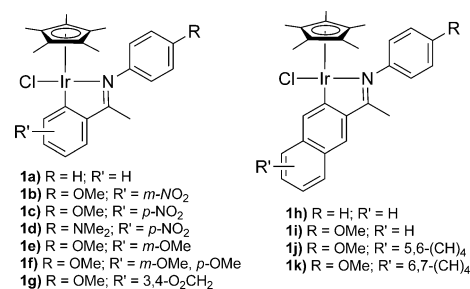
Figure 2. Cyclometalated \text{Ir}^{\text{III}} complexes examined in this study.
