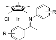
Figure 1. General structure of cyclometalated \text{Ir}^{\text{III}} complexes.
