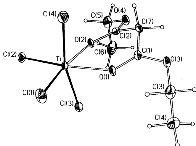
Fig. 1. Structure and numbering scheme of the [\text{CH}_2(\text{CO}_2\text{Et})_2\text{Cl}_4\text{Ti}] molecule.
