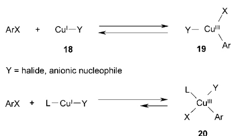
Scheme 6. Hypothesis of stabilization of the \text{Cu}^{\text{III}} oxidative addition product by the use of an appropriate supporting ligand L.
