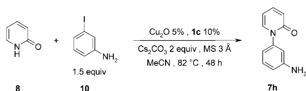
Scheme 2. Synthesis of the sedative Amphenidone 7h (Dornwall).
