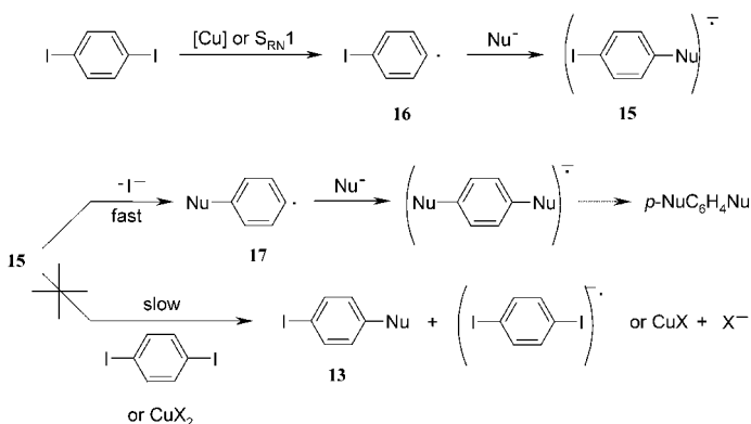
Scheme 4. Expected behavior of 1,4-diiodobenzene if mechanism would involve radical anion intermediates.
