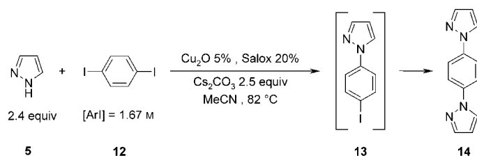
Scheme 3. Test for intermediacy of radical anion intermediates in Ullmann-type condensations.
