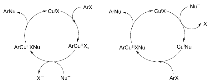
Scheme 5. The two alternative oxidative addition/reductive elimination mechanistic pathways for copper-catalyzed nucleophilic aromatic substitutions with aryl halides.
