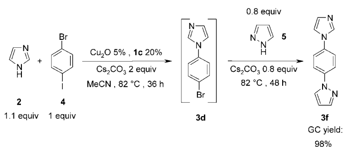
Scheme 1. One-pot synthesis of compound 3f starting from 4-bromiodobenzene.
