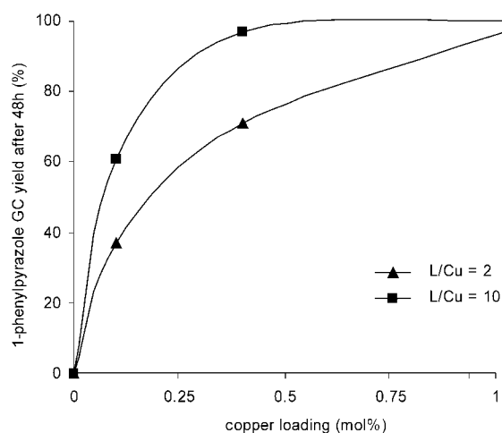
Figure 1. Beneficial use of a higher L/Cu ratio at low catalyst loading.
