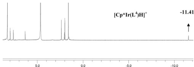
Figure 2. ^1\text{H} NMR spectrum ( \text{D}_2\text{O} solution) of a mixture of 19 and \text{HCOONH}_4 in 1:3 molar ratio at 296 K ( \text{pH} \approx 7 ).
