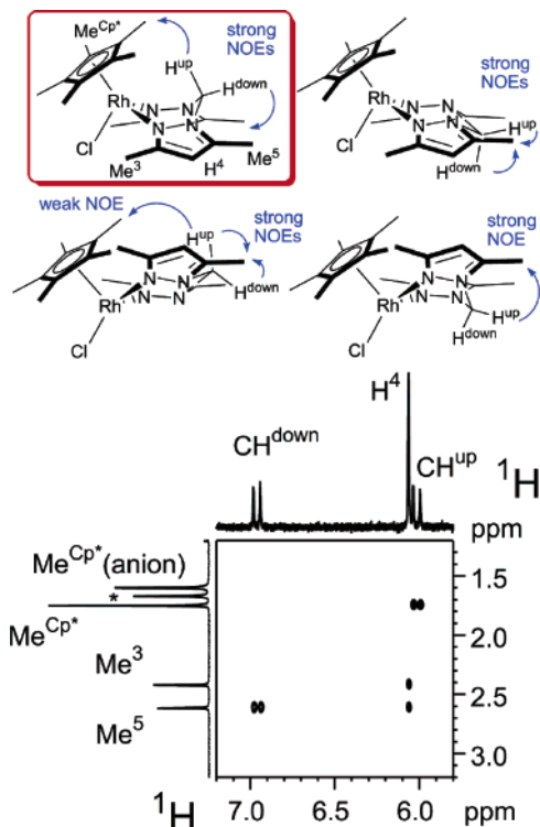
Figure 1. Section of ^1\text{H} -NOESY NMR spectrum (400.13 MHz, 296 K, \text{CD}_2\text{Cl}_2 , mixing time = 800 ms) of complex 5 . On the top, the two boat and chair conformations of the metallacycle \text{M}(\text{N}-\text{N})_2\text{C} are depicted with the expected NOEs between \text{CH}^{\text{up}} (and \text{CH}^{\text{down}} ) and \text{Me}^5 (and \text{Me}^{\text{Cp*}} ). The asterisk (*) denotes the resonance of \text{H}_2\text{O} .
