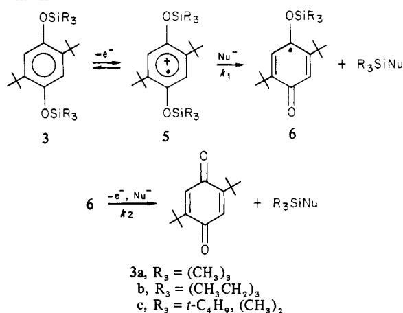
Scheme II
