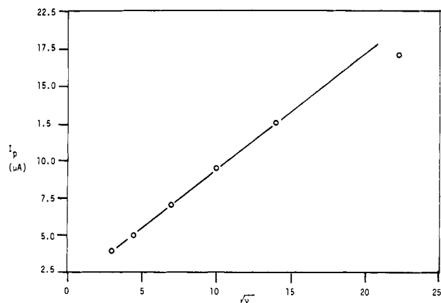
Figure 1. Peak current ( I_p ) as a function of scan rate for 4.8 mM 3a in \text{H}_2\text{CCl}_2 , 0.2 M \text{Bu}_4\text{NClO}_4 .
