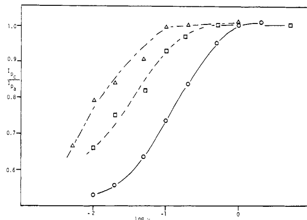
Figure 3. Ratio of cathodic to anodic peak currents as a function of sweep rate ( \nu ) for compounds 3a , \circ ; 3b , \square ; 3c , \Delta .
