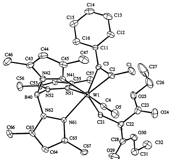
Fig. 3. ORTEP of \text{Tp}'(\text{CO})(\text{PhCCMe})\text{WCH}_2\text{CH}(\text{COOEt})_2 ( 6 ).
