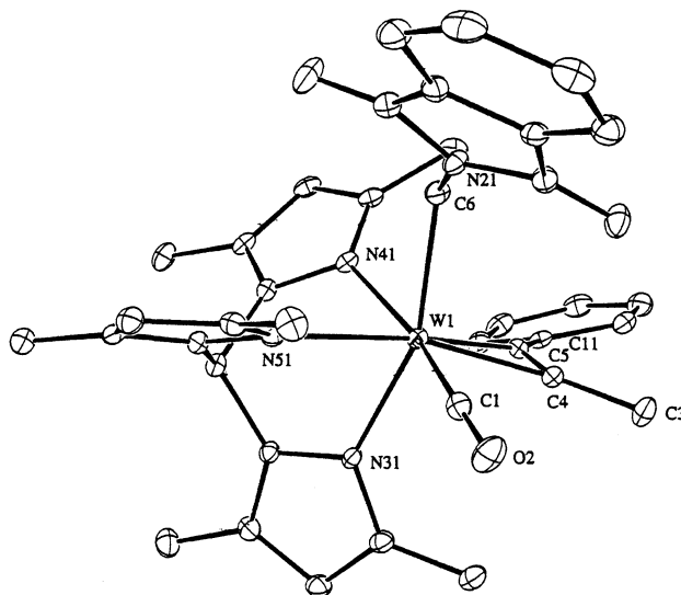
Fig. 2. ORTEP diagram of \text{Tp}'(\text{CO})(\text{PhCCMe})\text{W}-\text{CH}_2 -phthalimide ( 5 ).
