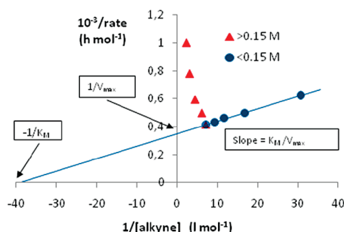
Figure 4. Lineweaver–Burke plot: 1/[alkyne] vs 1/rate. Circles represent values at [alkyne] < 0.15 M, triangles represent values at [alkyne] > 0.15 M.
