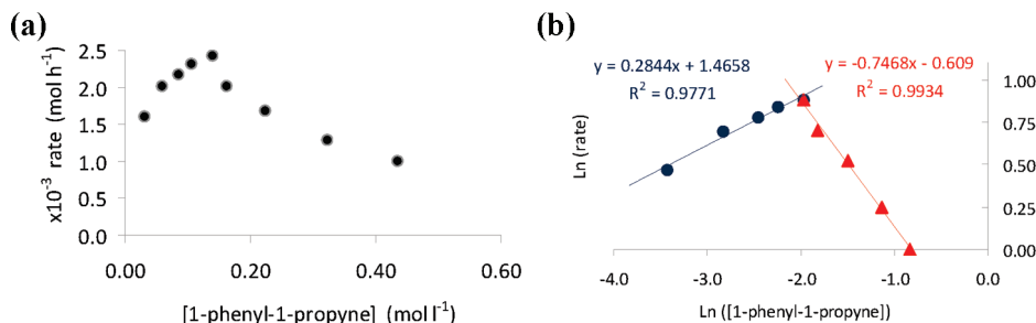
Figure 3. (a) Plot of rate of hydrogenation versus substrate concentration. (b) Plot of ln(rate) versus ln[1-phenyl-1-propyne]; circles represent values at [alkyne] < 0.15 M, triangles represent values at [alkyne] > 0.15 M.
