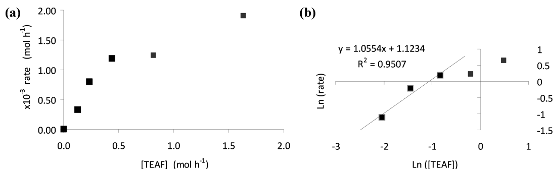
Figure 2. (a) Plot of rate of hydrogenation versus hydrogen donor concentration. (b) Plot of ln(rate) versus ln[TEAF].
