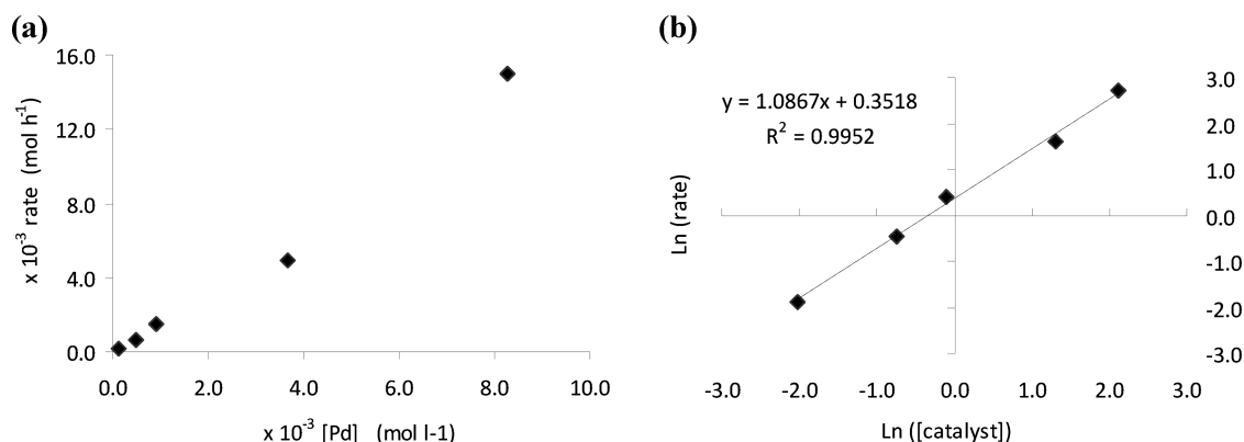
Figure 1. (a) Plot of rate of hydrogenation versus catalyst concentration. (b) Plot of ln(rate) versus ln[catalyst].
