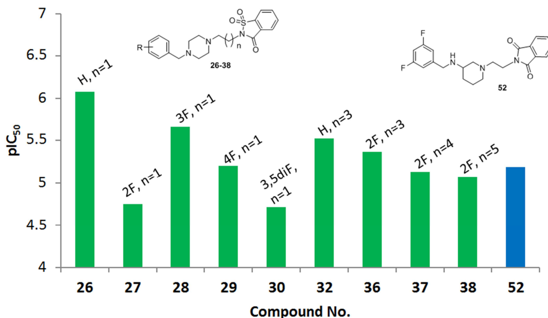
Figure 3. Comparison of EeAChE pIC 50 values of the most active compounds.
