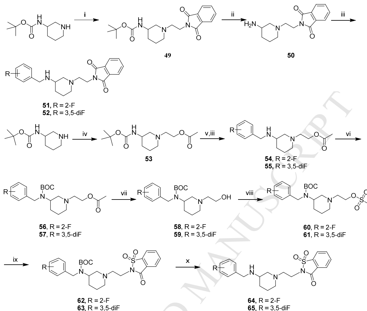
Scheme 2. Synthesis of compounds 51 , 52 , 64 and 65 . Reagents and conditions: i) 2-(2-bromoethyl)isoindoline-1,3-dione, acetonitrile, K_2CO_3 , NaI, 80 °C, 24 h, ii) TFA, dichloromethane, R.T., 4 h, iii) 1-(chloromethyl)-2-fluorobenzene/1-(bromomethyl)-3,5-difluorobenzene, acetonitrile, K_2CO_3 , 80 °C, 24 h, iv) 2-bromoethyl acetate, acetonitrile, K_2CO_3 , 80 °C, 24 h; v) TFA, dichloromethane, R.T., 2 h; vi) di- tert -butyl dicarbonate, TEA, dichloromethane, R.T., 2 h; vii) methanol-water mixture, K_2CO_3 , 65 °C, 2 h, viii) methanesulfonyl chloride, dichloromethane, TEA, R.T., 2 h; ix) sodium saccharin, acetonitrile, K_2CO_3 , 80 °C, 24 h; x) 1M HCl in ethyl acetate, R.T., 24 h.
