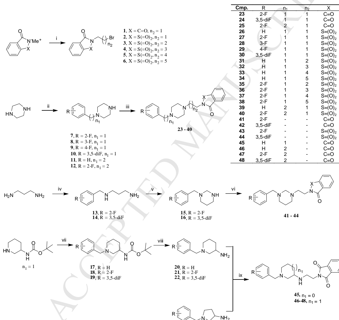
Scheme 1. Synthesis of compounds 23–48 . Reagents and conditions: i) \alpha,\omega -dibromoalkane, acetonitrile, K 2 CO 3 , 80 °C, 24 h; ii) phenyl-alkyl-halide derivative, acetonitrile, R.T., 24 h; iii) compounds 1–6 , acetonitrile, K 2 CO 3 , 80 °C, 24 h; iv) 1-(chloromethyl)-2-fluorobenzene/1-(bromomethyl)-3,5-difluorobenzene, acetonitrile, 0 °C/R.T., 20 h; v) formaldehyde, acetonitrile/water, R.T., 1 h; vi) compounds 1 or 2 , DMF, K 2 CO 3 , 110 °C, 24
