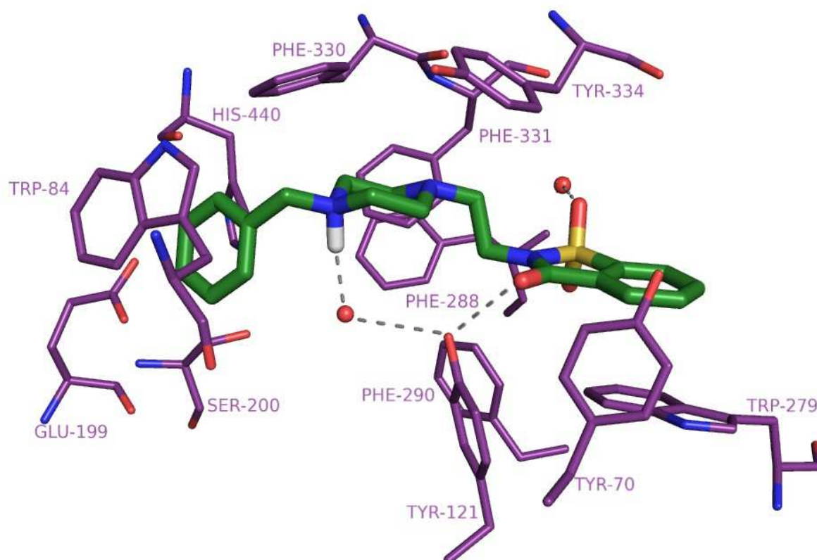
Figure 5. The binding mode of compound 26 within the active site of AChE. The red spheres represent conserved water molecules engaged in the hydrogen bond network. Hydrogen bonds marked by grey dotted line.
