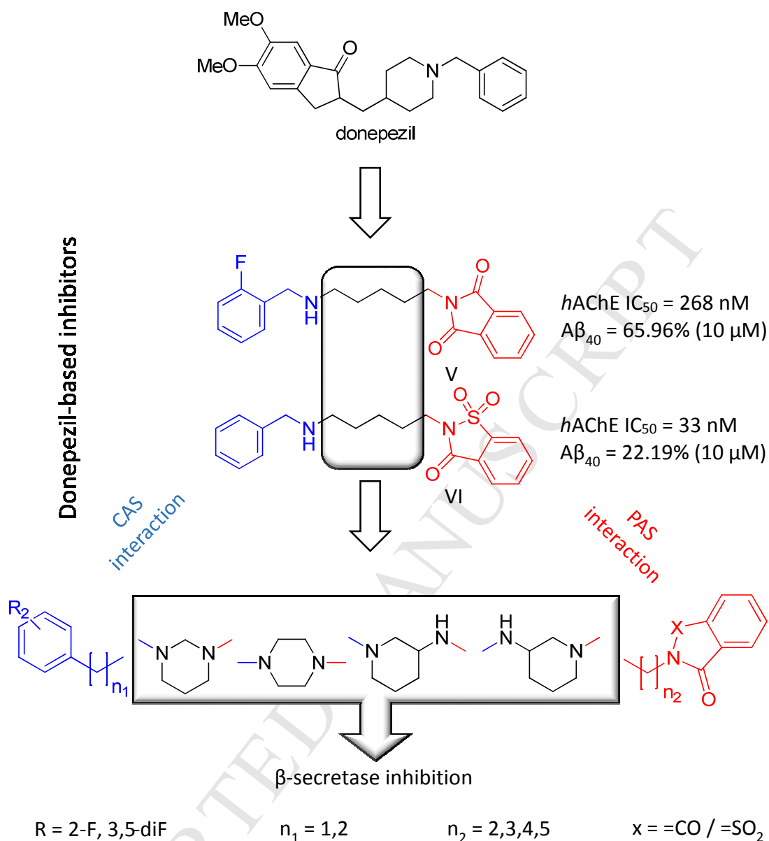
Figure 2. Design strategy of new phthalimide and saccharin derivatives with alicyclic amines targeting cholinesterases, BACE1 and A \beta aggregation.
