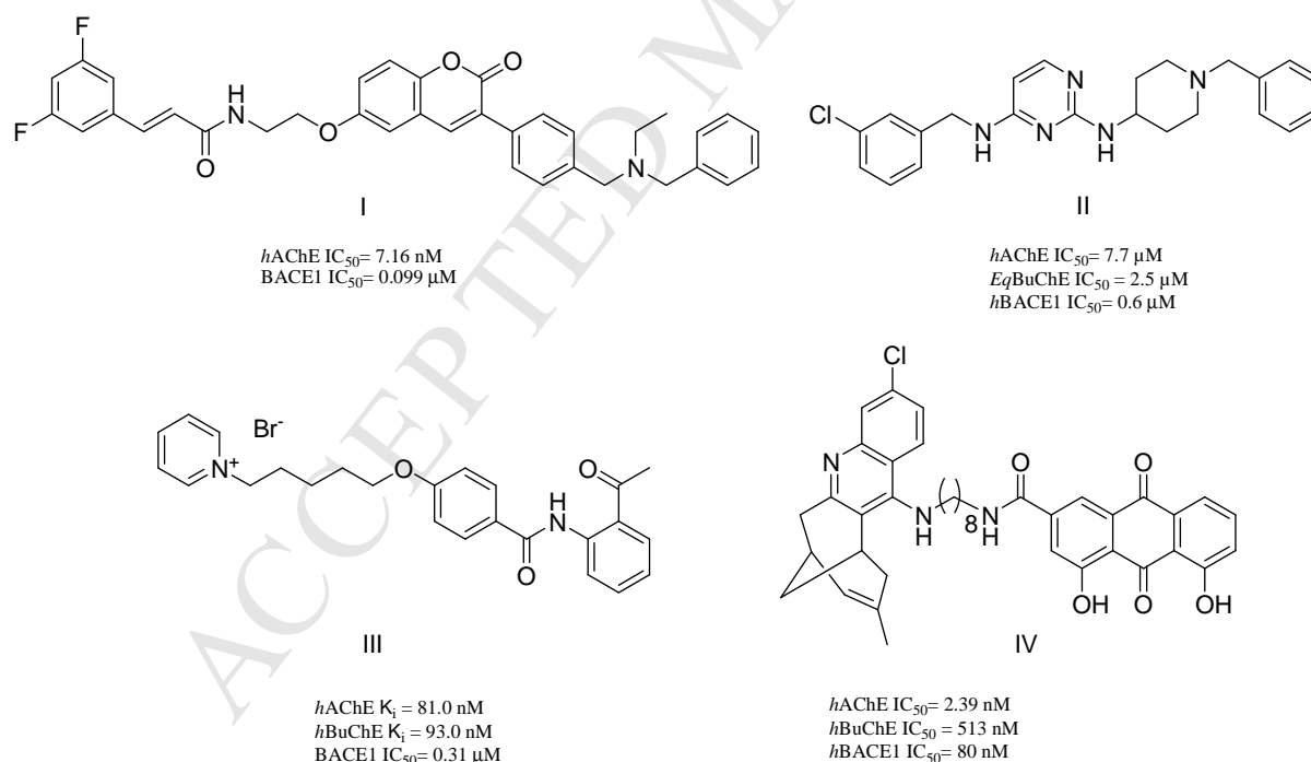
Figure 1. Previously described, selected MTDLs, inhibitors of AChE and BACE1.
