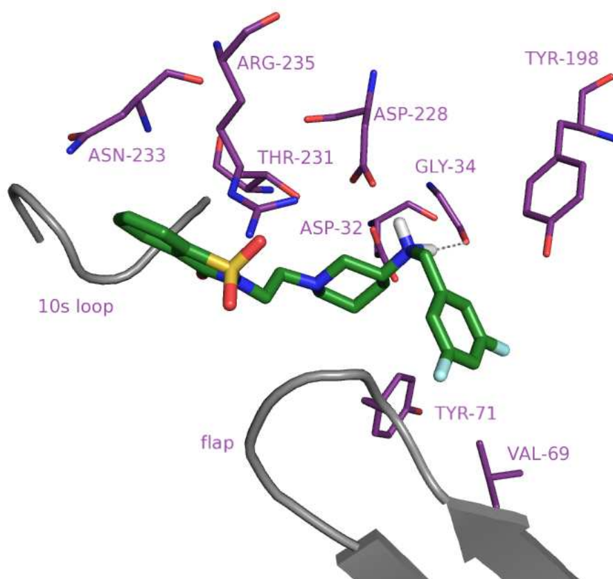
Figure 6. The binding mode of compound 65 within the active site of BACE1. Asp32 and Asp228 constitute catalytic dyad. The 10s loop and flap are the most flexible parts of BACE1. The S2' pocket contains Tyr71, Val69 and Tyr198. Asn233 and Arg235 belong to the S2 site, and Thr231 to the S3 pocket. Hydrogen bonds marked by grey dotted line.
