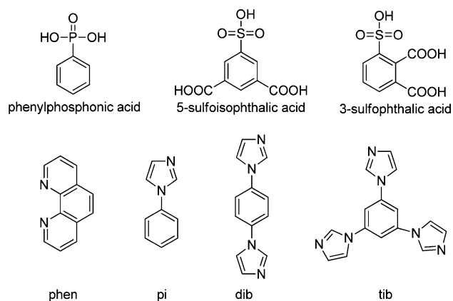
Scheme 1. Schematic Representation of the Ligands
