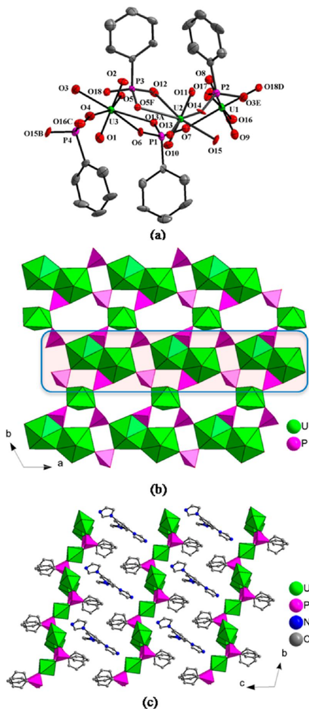
Figure 1. (a) ORTEP representation of the coordination environment in UPhP-1. Thermal ellipsoids are drawn at the 50% probability level. Symmetry code: A, x, -1 + y, z ; B, -1 + x, -1 + y, z ; C, -1 + x, y, z ; D, 1 + x, y, z ; E, 1 + x, 1 + y, z ; F, x, 1 + y, z . (b) The layer of UPhP-1 contains the chain in highlight. (c) The layers stack along the [100] direction.
