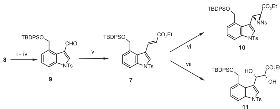
Scheme 2. Synthesis of 7 and further transformations. Reagents: (i) \text{LiAlH}_4 , THF, rt, 12 h, 94%; (ii) imidazole (3.0 equiv), TBDPSCl (1.7 equiv), DMF, 0 °C then rt, 12 h, 85%; (iii) DMF (3.5 equiv), \text{POCl}_3 (1.1 equiv), DMF, 0 °C then rt, 12 h, 78%; (iv) TsCl (1.5 equiv), \text{NEt}_3 (1.5 equiv), DCM, 12 h, 97%; (v) (\text{EtO})_2\text{P}(\text{O})\text{CH}_2\text{CO}_2\text{Et} (2.4 equiv), LiCl (2.4 equiv), DBU (2.0 equiv), MeCN, 24 h, 83%; (vi) PhINNs (0.67 equiv), (+)-2,2'-isopropylidenebis[(4 R )-4-phenyl-2-oxazoline] (0.067 equiv), \text{Cu}(\text{OTf})_2 (0.033 equiv), DCM, rt, 12 h; (vii) methane sulfonamide (3 equiv), AD-mix alpha (0.01 equiv \text{K}_2\text{Os}_2\text{O}_2(\text{OH})_4 ), ^t\text{BuOH} , \text{H}_2\text{O} , 24 h, rt.
