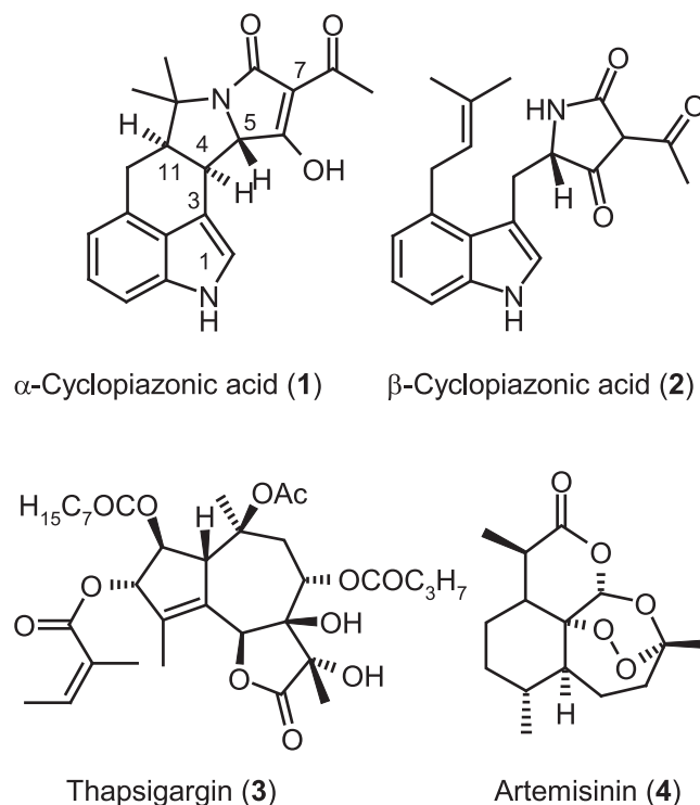
Figure 1. Known inhibitors of SERCA.
