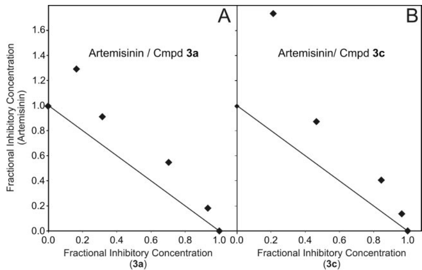
FIG. 2. Interaction of artemisinin and two novel endoperoxides in inhibiting parasite growth. Isobolograms were constructed from the IC 50 values in Table 2. For each drug combination, FICs were calculated by dividing the measured apparent IC 50 values for the individual drugs in the different combinations of artemisinin with compound (Cmpd) 3a (A) or compound 3c (B) by the IC 50 values obtained when the drugs were used alone.
