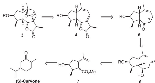
Scheme 1. Retrosynthetic Analysis of Guaianolide-Endoperoxide
