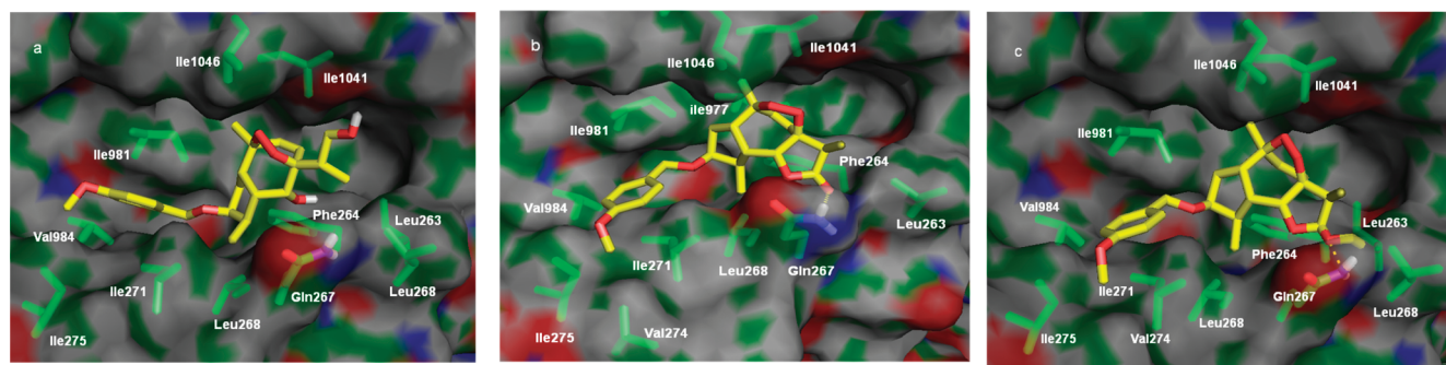
Figure 2. Docking pose of (a) 13 , (b) 3 , (c) 22 in the homology model of PfSERCA. Only side chain atoms of key residues of the active site are shown for clarity. Figures were created using PyMOL1.1 (The PyMOL Molecular Graphics System, version 1.1, Schrodinger, LLC).
