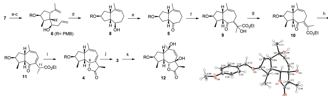
Scheme 2. Stereoselective Synthesis of Thaperoxide 3 a
