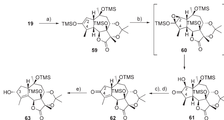
Scheme 8. Enone formation, part I. a) \text{TMSCl} , \text{Et}_3\text{N} , DMF, 130 °C, 43 h; b) DMDO, \text{Me}_2\text{CO} , \text{CH}_2\text{Cl}_2 , –78 °C for 30 min, then RT for 40 min, 87 % over two steps; c) \text{TMSCl} , \text{Et}_3\text{N} , DMF, 150 °C, 90 %; d) \text{PhSeBr} , \text{CH}_2\text{Cl}_2 , 0 °C to RT, 94 %; e) \text{NaBH}_4 , MeOH, 0 °C, 86 %, dr 4:1 ( R/S at C-3) (TMS=trimethylsilyl, DMDO=dimethyldioxirane).
