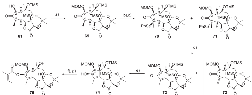
Scheme 11. Enone formation, part II. a) MOMCl, Hünig's base, CH 2 Cl 2 , RT, 18 h, 88 %; b) NaHMDS, THF, -78 to -20 °C then TMSCl at -78 °C; c) PhSeCl, CH 2 Cl 2 , -78 °C, 2 h; d) O 3 , -78 °C, 2 min then diisopropylamine, -78 °C to RT, 37 % 73 over three steps; e) NaBH 4 , THF, RT, 19 h, 99 % (dr >19:1); f) TBAF, THF, 0 °C to RT, 35 min; g) 2,4,6-trichlorobenzoyl chloride, Et 3 N, PhMe, angelic acid, 75 °C, 2 d, 48 % over two steps (HMDS=bis(trimethylsilyl)amide).
