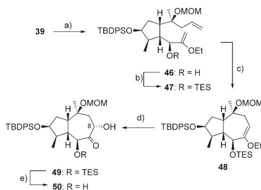
Scheme 6. Formation of bicyclic intermediate 49 . a) Ethyl vinyl ether, t BuLi, THF, –78°C, 90 min; b) TESCl, imidazole, DMAP, DMF, RT, 19 h, 86% over three steps from alcohol 38s ; c) Grubbs' second generation catalyst, CH 2 Cl 2 , reflux, 21 h, 88%; d) AD-mix \alpha , NaHCO 3 , MeSO 2 NH 2 , t BuOH, H 2 O, RT, 15 h, 96%; e) TBAF, THF, 0°C, 20 min (TES=triethylsilyl).
