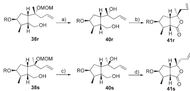
Scheme 4. Synthesis of lactones 41s and 41r ( R = TBDPS). a) PPTS, MeOH, RT, 34%; b) cat. TPAP, NMO, 4 Å molecular sieves, \text{CH}_2\text{Cl}_2 , RT, 76%; c) PPTS, MeOH, RT, 32%; d) cat. TPAP, NMO, 4 Å molecular sieves, \text{CH}_2\text{Cl}_2 , RT, 92% (TPAP = tetra- n -propylammonium perruthenate).
