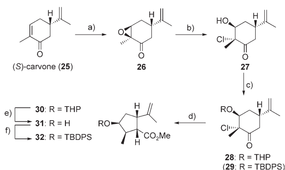
Scheme 2. Generation of cyclopentane fragment 32 . a) H 2 O 2 , MeOH, NaOH, RT, 3 h; b) TFA, THF, LiCl, 0 °C, 90 min, 98 % over two steps; c) 2,3-dihydropyran, PPTS, CH 2 Cl 2 , RT, 17 h, 84 %; d) NaOMe, MeOH, Et 2 O, 0 °C, 1 h; e) MeOH, PPTS, 50 °C, 15 h; f) TBDPSCI, imidazole, DMAP, DMF, RT, 16 h, 84 % over three steps (TFA = trifluoroacetic acid, THF = tetrahydrofuran, PPTS = pyridinium para -toluenesulfonate, TBDPS = tert -butyldiphenylsilyl, THP = tetrahydropyran-2-yl).
