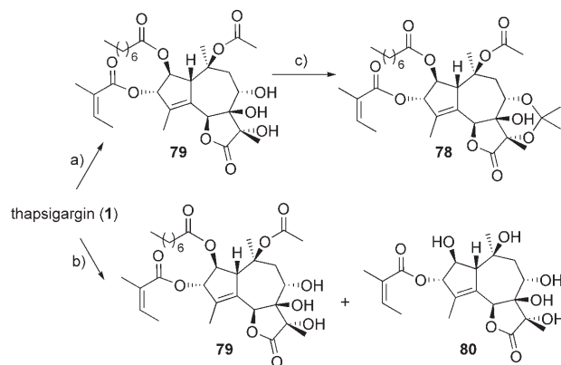
Scheme 13. Known transformations of thapsigargin. a) Et 3 N, MeOH, RT, 7 h, 99%; [8] b) Et 3 N, MeOH, 75 °C, 48 h, 47% 79 + 48% 80 ; [59] c) 2,2-dimethoxypropane, Me 2 CO, p TsOH, RT, 3 h (yield not reported). [6]
